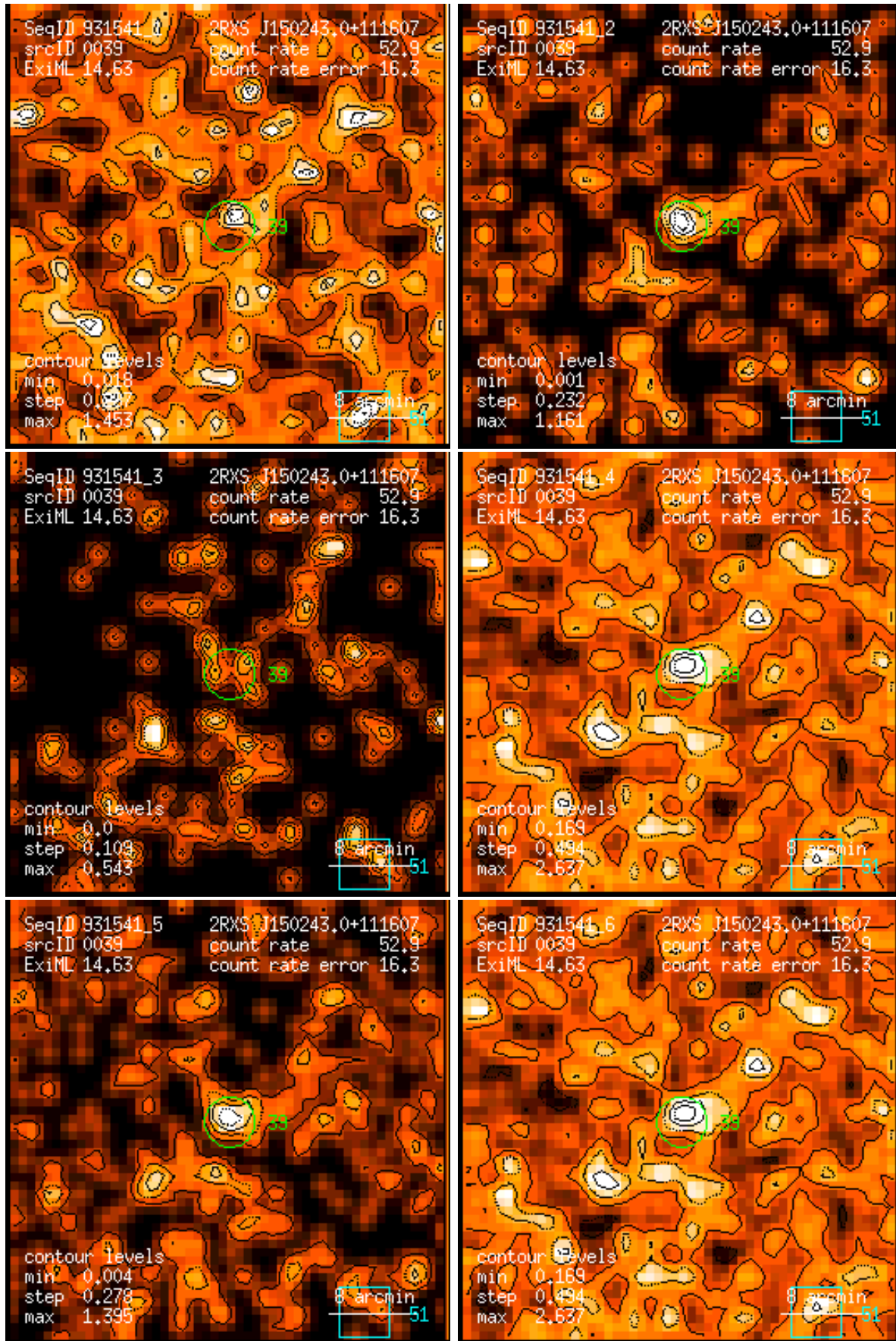
Figure 39: RASS 931541: detection 0039: band rate images, Gaussian filter: (1) PSPC channels 11 – 41, (2) 52 – 90, (3) 91 – 201, (4) 11 – 235, (5) 52 – 201, (6) 11 – 201. Broad band rates in counts/ks. Band rate contour levels in counts/ks/arcmin 2 .
