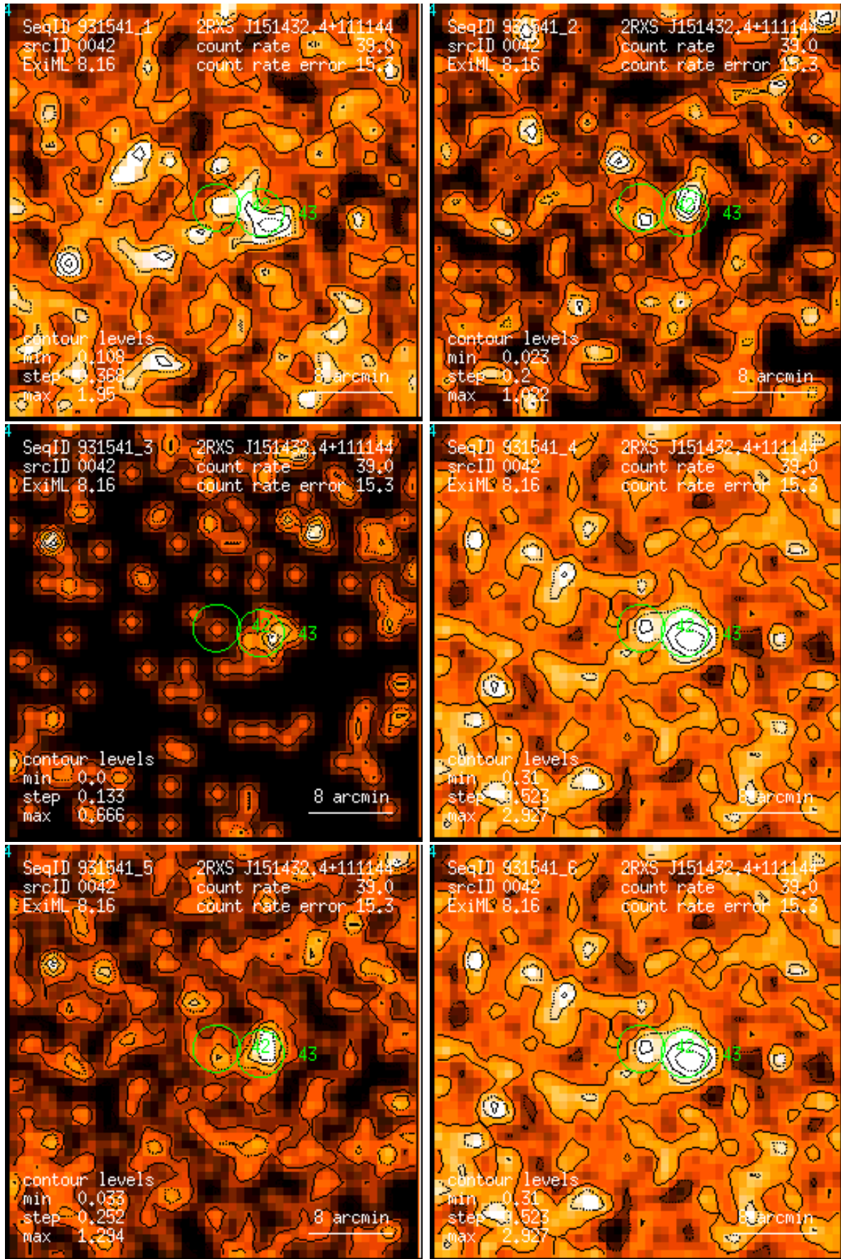
Figure 42: RASS 931541: detection 0042: band rate images, Gaussian filter: (1) PSPC channels 11 – 41, (2) 52 – 90, (3) 91 – 201, (4) 11 – 235, (5) 52 – 201, (6) 11 – 201. Broad band rates in counts/ks. Band rate contour levels in counts/ks/arcmin 2 .
