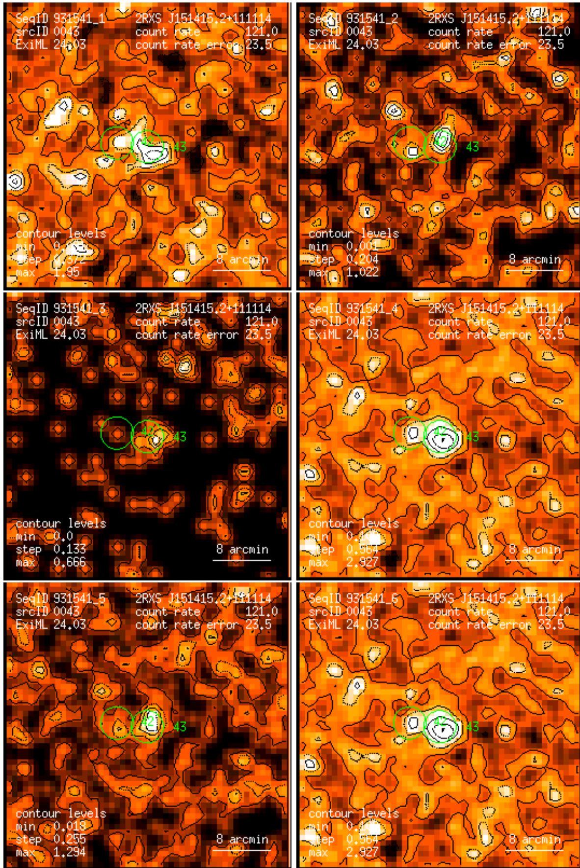
Figure 43: RASS 931541: detection 0043: band rate images, Gaussian filter: (1) PSPC channels 11 – 41, (2) 52 – 90, (3) 91 – 201, (4) 11 – 235, (5) 52 – 201, (6) 11 – 201. Broad band rates in counts/ks. Band rate contour levels in counts/ks/arcmin 2 .
