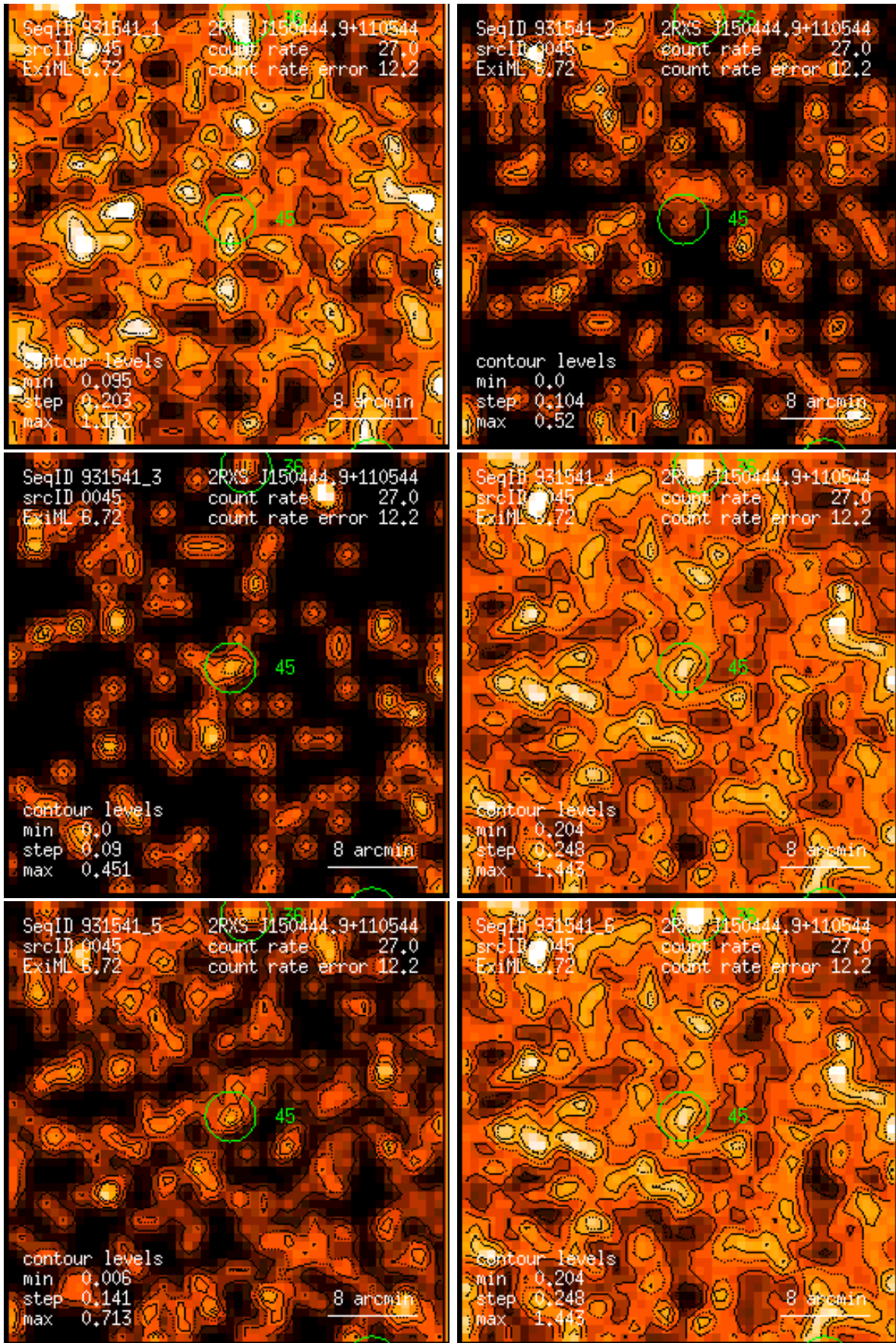
Figure 45: RASS 931541: detection 0045: band rate images, Gaussian filter: (1) PSPC channels 11 – 41, (2) 52 – 90, (3) 91 – 201, (4) 11 – 235, (5) 52 – 201, (6) 11 – 201. Broad band rates in counts/ks. Band rate contour levels in counts/ks/arcmin 2 .
