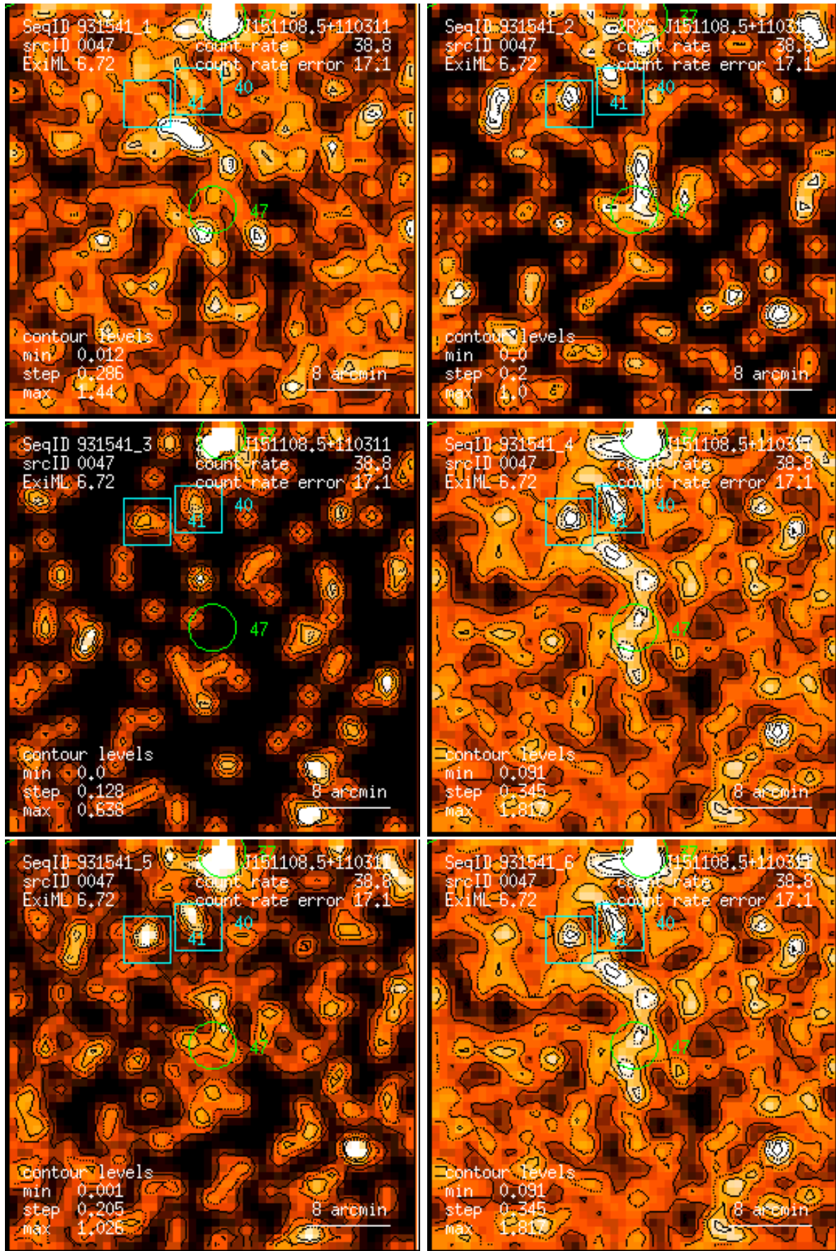
Figure 47: RASS 931541: detection 0047: band rate images, Gaussian filter: (1) PSPC channels 11 – 41, (2) 52 – 90, (3) 91 – 201, (4) 11 – 235, (5) 52 – 201, (6) 11 – 201. Broad band rates in counts/ks. Band rate contour levels in counts/ks/arcmin 2 .
