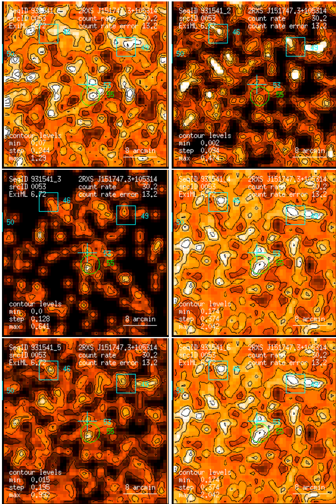
Figure 53: RASS 931541: detection 0053: band rate images, Gaussian filter: (1) PSPC channels 11 – 41, (2) 52 – 90, (3) 91 – 201, (4) 11 – 235, (5) 52 – 201, (6) 11 – 201. Broad band rates in counts/ks. Band rate contour levels in counts/ks/arcmin 2 .
