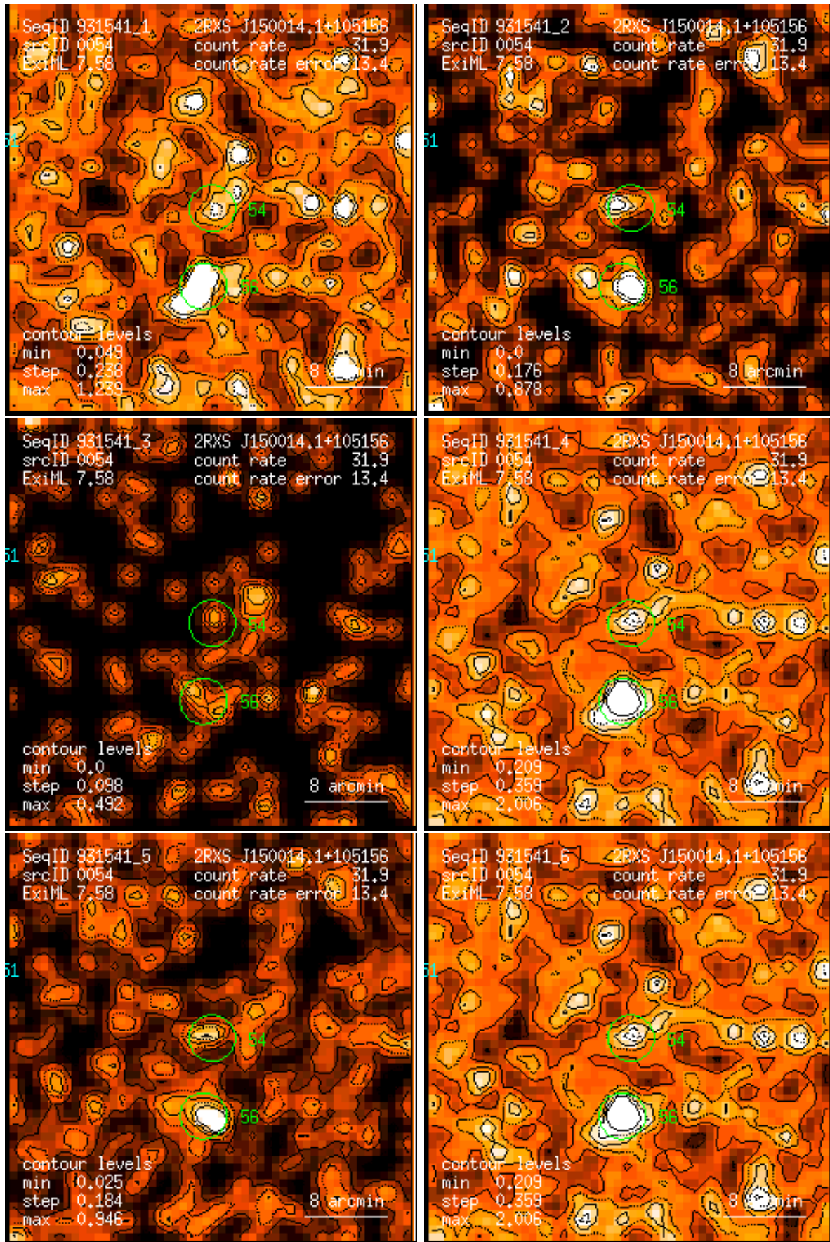
Figure 54: RASS 931541: detection 0054: band rate images, Gaussian filter: (1) PSPC channels 11 – 41, (2) 52 – 90, (3) 91 – 201, (4) 11 – 235, (5) 52 – 201, (6) 11 – 201. Broad band rates in counts/ks. Band rate contour levels in counts/ks/arcmin 2 .
