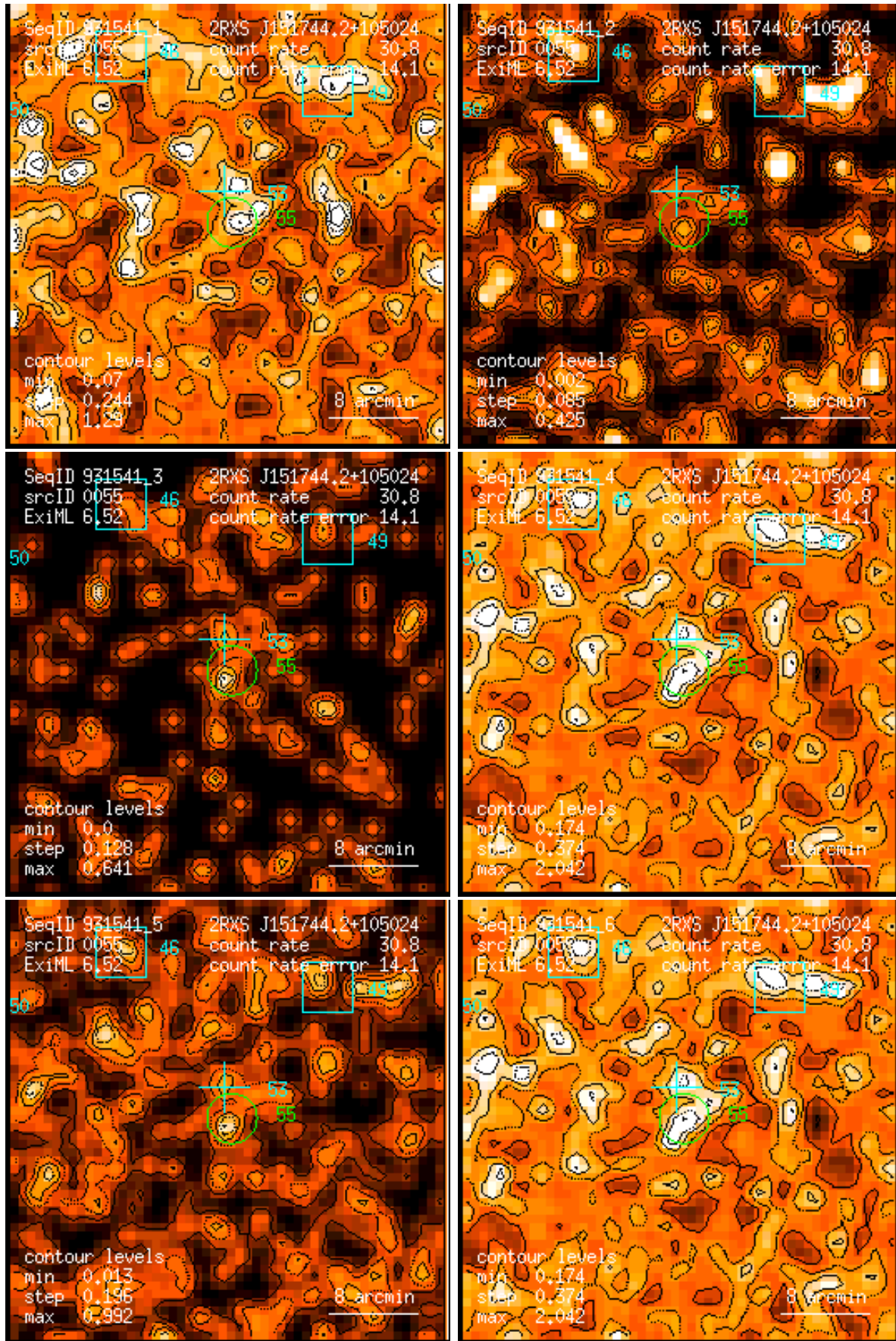
Figure 55: RASS 931541: detection 0055: band rate images, Gaussian filter: (1) PSPC channels 11 – 41, (2) 52 – 90, (3) 91 – 201, (4) 11 – 235, (5) 52 – 201, (6) 11 – 201. Broad band rates in counts/ks. Band rate contour levels in counts/ks/arcmin 2 .
