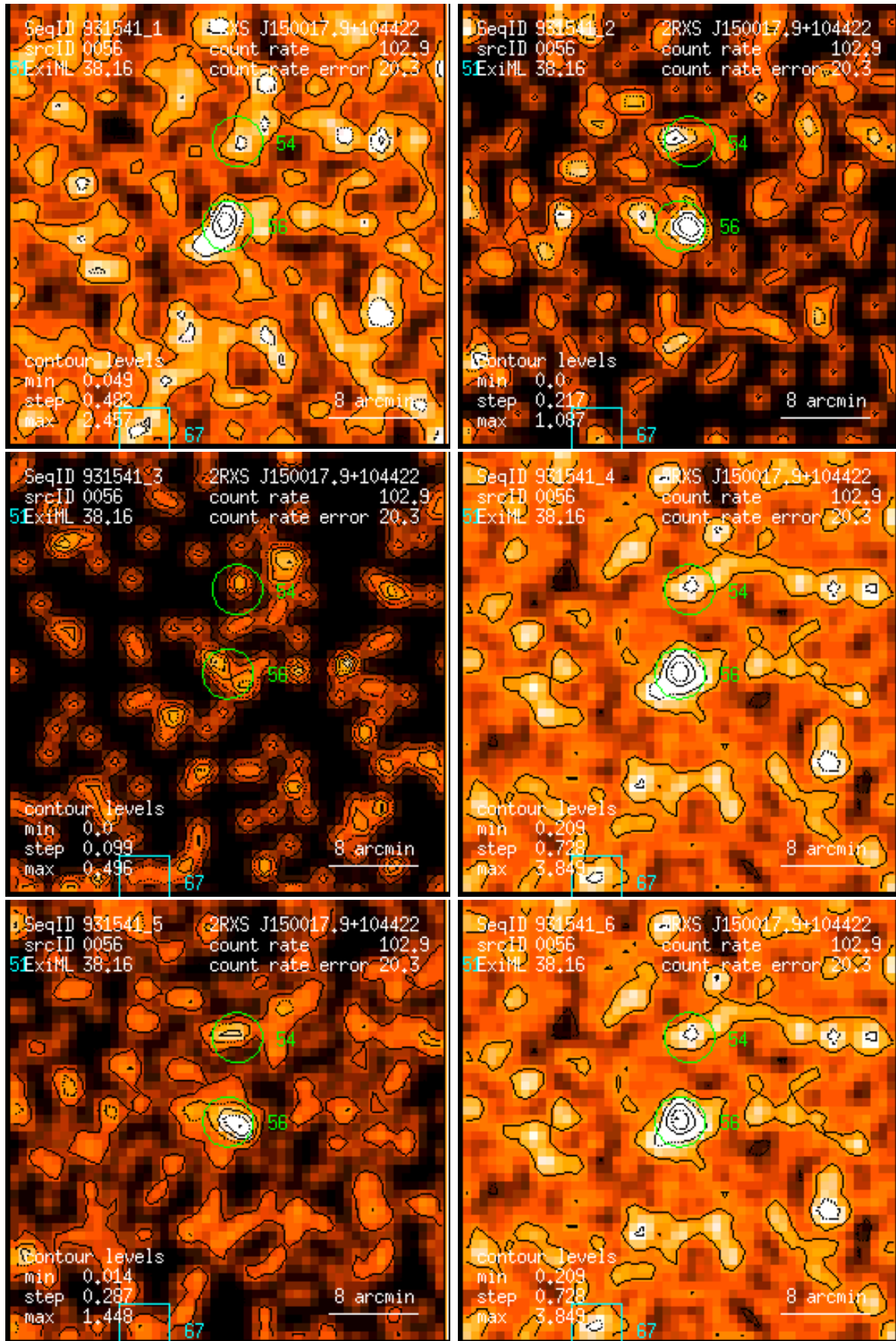
Figure 56: RASS 931541: detection 0056: band rate images, Gaussian filter: (1) PSPC channels 11 – 41, (2) 52 – 90, (3) 91 – 201, (4) 11 – 235, (5) 52 – 201, (6) 11 – 201. Broad band rates in counts/ks. Band rate contour levels in counts/ks/arcmin 2 .
