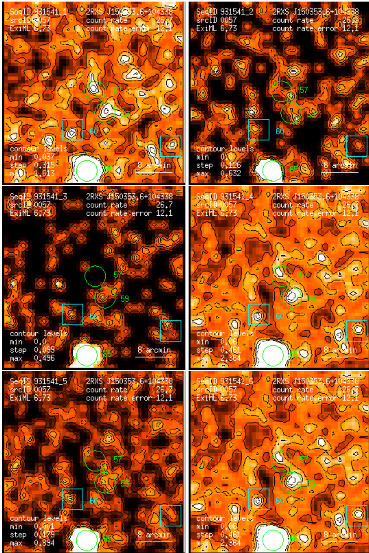
Figure 57: RASS 931541: detection 0057: band rate images, Gaussian filter: (1) PSPC channels 11 – 41, (2) 52 – 90, (3) 91 – 201, (4) 11 – 235, (5) 52 – 201, (6) 11 – 201. Broad band rates in counts/ks. Band rate contour levels in counts/ks/arcmin 2 .
