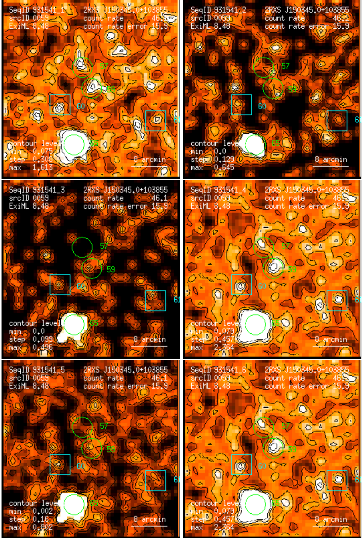
Figure 59: RASS 931541: detection 0059: band rate images, Gaussian filter: (1) PSPC channels 11 – 41, (2) 52 – 90, (3) 91 – 201, (4) 11 – 235, (5) 52 – 201, (6) 11 – 201. Broad band rates in counts/ks. Band rate contour levels in counts/ks/arcmin 2 .
