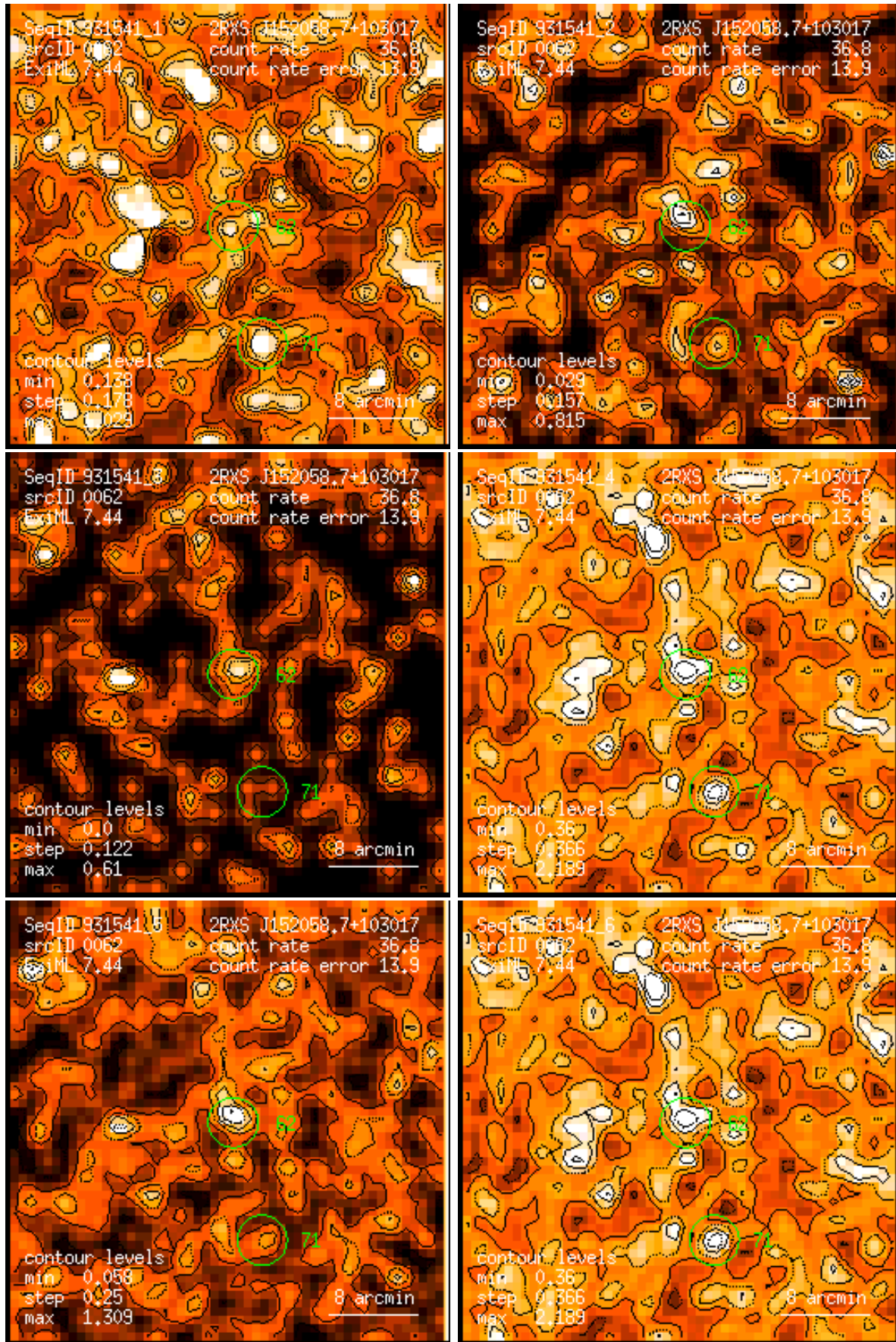
Figure 62: RASS 931541: detection 0062: band rate images, Gaussian filter: (1) PSPC channels 11 – 41, (2) 52 – 90, (3) 91 – 201, (4) 11 – 235, (5) 52 – 201, (6) 11 – 201. Broad band rates in counts/ks. Band rate contour levels in counts/ks/arcmin 2 .
