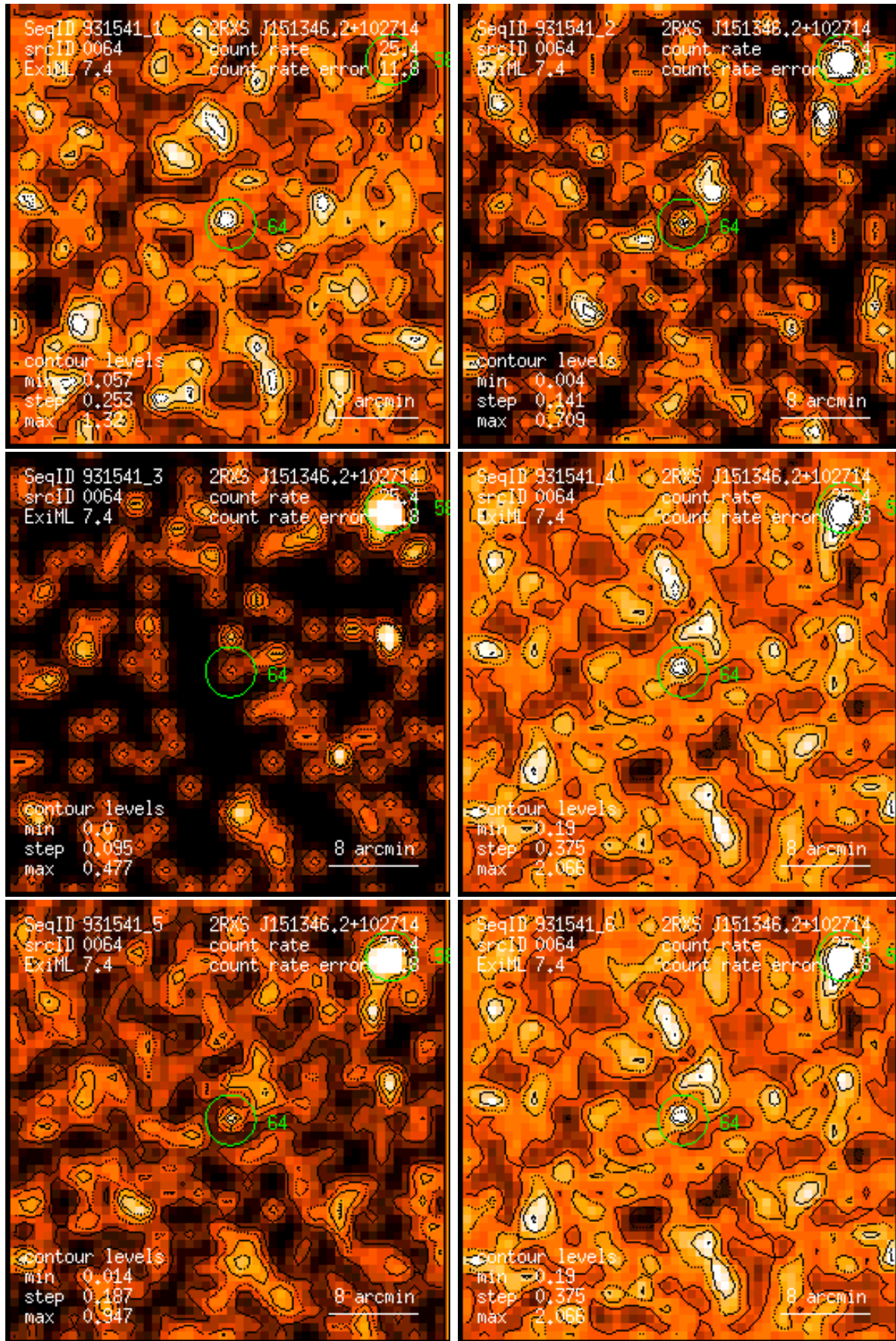
Figure 64: RASS 931541: detection 0064: band rate images, Gaussian filter: (1) PSPC channels 11 – 41, (2) 52 – 90, (3) 91 – 201, (4) 11 – 235, (5) 52 – 201, (6) 11 – 201. Broad band rates in counts/ks. Band rate contour levels in counts/ks/arcmin 2 .
