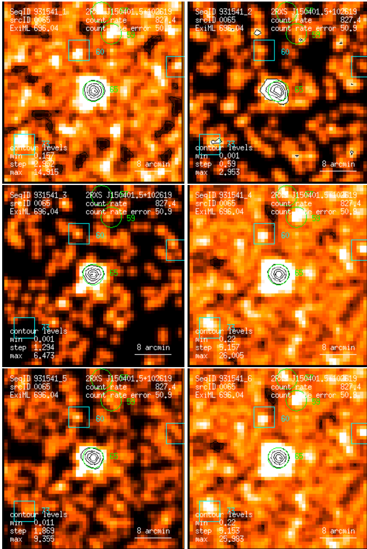
Figure 65: RASS 931541: detection 0065: band rate images, Gaussian filter: (1) PSPC channels 11 – 41, (2) 52 – 90, (3) 91 – 201, (4) 11 – 235, (5) 52 – 201, (6) 11 – 201. Broad band rates in counts/ks. Band rate contour levels in counts/ks/arcmin 2 .
