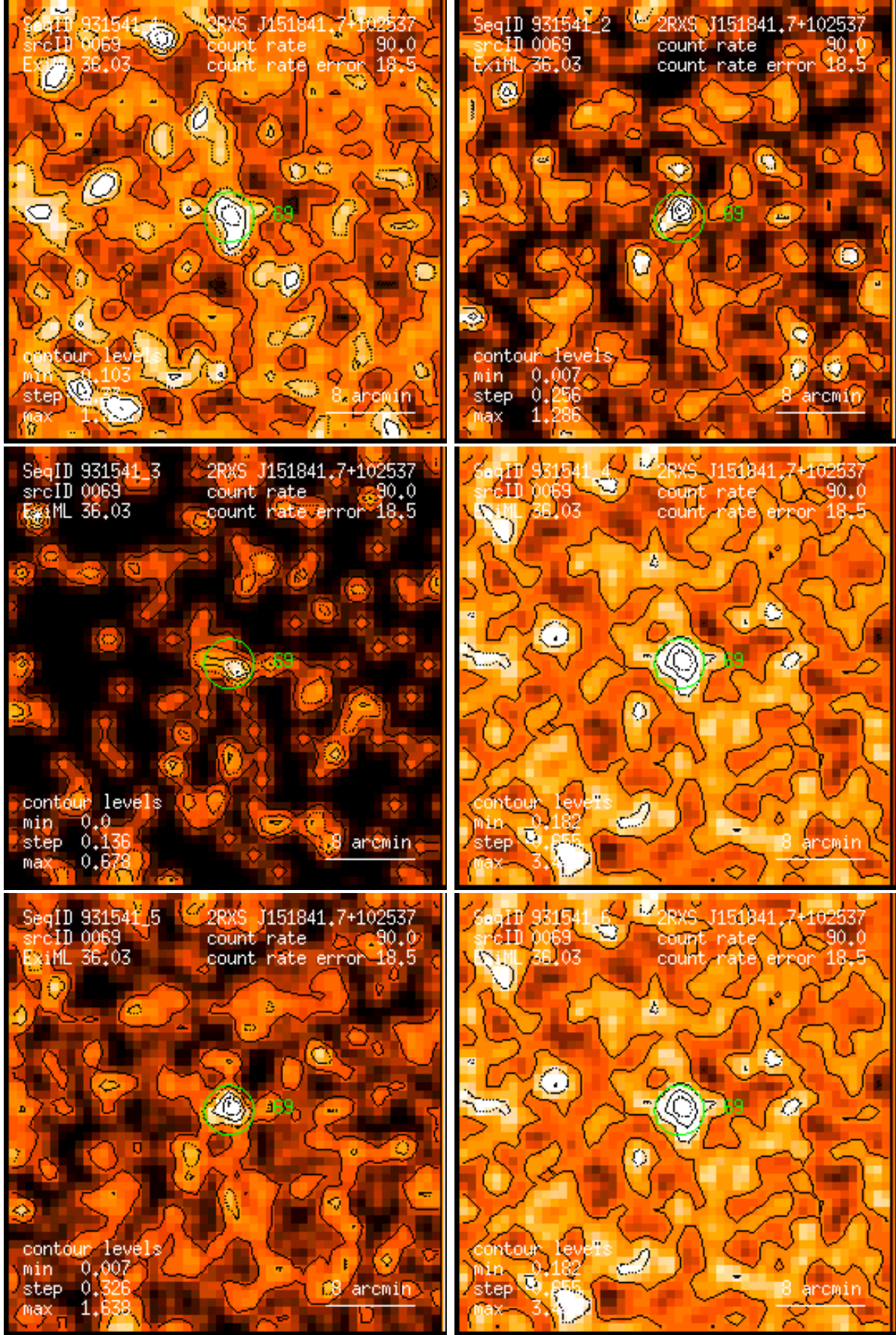
Figure 69: RASS 931541: detection 0069: band rate images, Gaussian filter: (1) PSPC channels 11 – 41, (2) 52 – 90, (3) 91 – 201, (4) 11 – 235, (5) 52 – 201, (6) 11 – 201. Broad band rates in counts/ks. Band rate contour levels in counts/ks/arcmin 2 .
