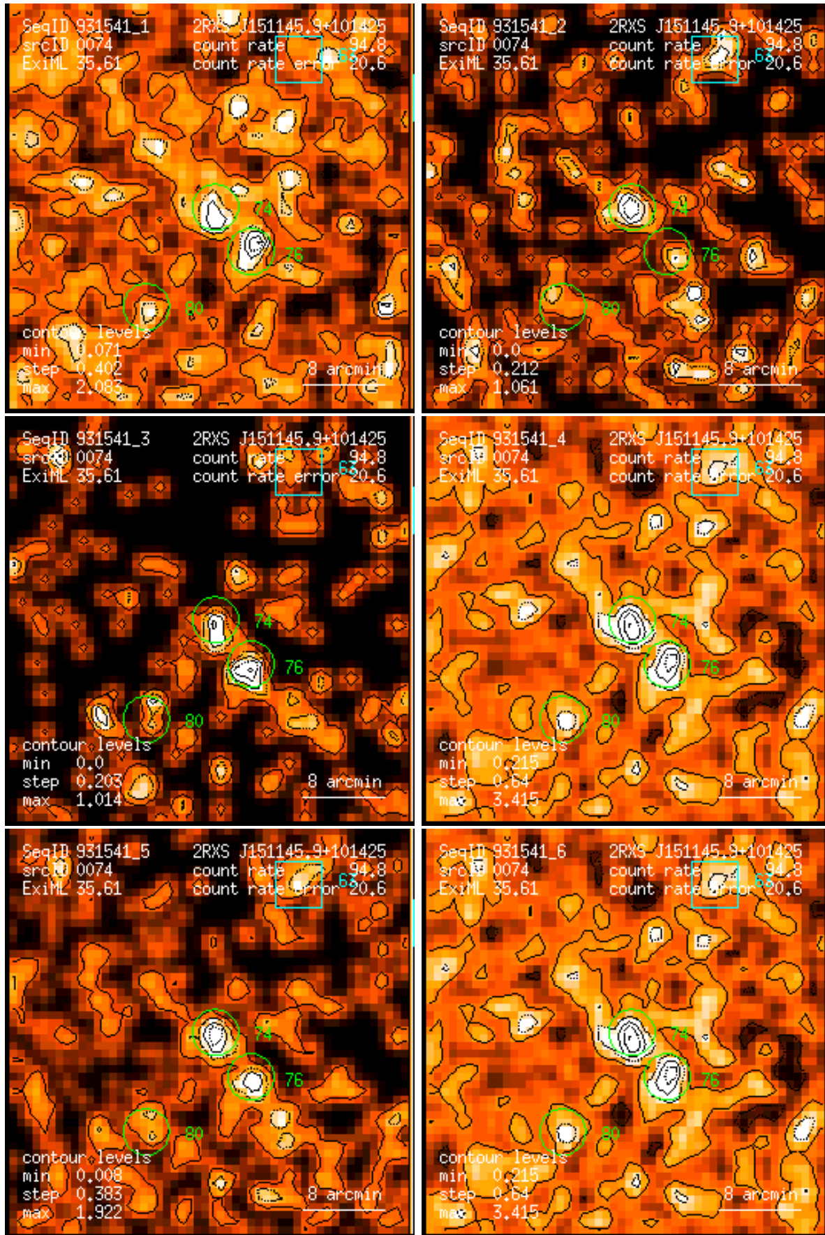
Figure 74: RASS 931541: detection 0074: band rate images, Gaussian filter: (1) PSPC channels 11 – 41, (2) 52 – 90, (3) 91 – 201, (4) 11 – 235, (5) 52 – 201, (6) 11 – 201. Broad band rates in counts/ks. Band rate contour levels in counts/ks/arcmin 2 .
