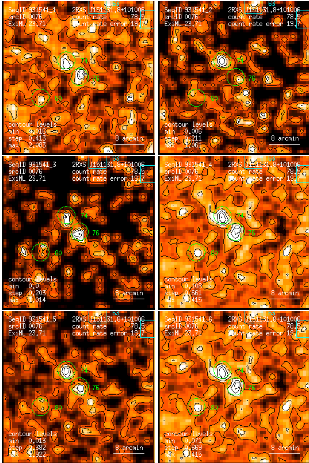
Figure 76: RASS 931541: detection 0076: band rate images, Gaussian filter: (1) PSPC channels 11 – 41, (2) 52 – 90, (3) 91 – 201, (4) 11 – 235, (5) 52 – 201, (6) 11 – 201. Broad band rates in counts/ks. Band rate contour levels in counts/ks/arcmin 2 .
