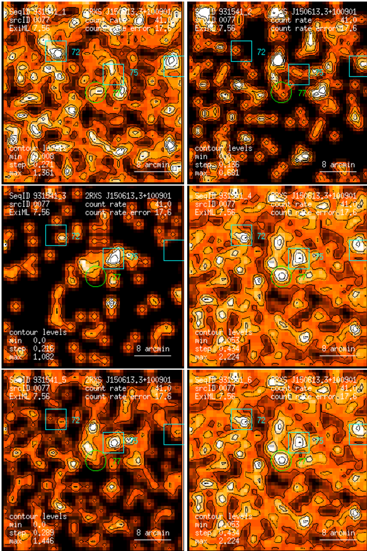
Figure 77: RASS 931541: detection 0077: band rate images, Gaussian filter: (1) PSPC channels 11 – 41, (2) 52 – 90, (3) 91 – 201, (4) 11 – 235, (5) 52 – 201, (6) 11 – 201. Broad band rates in counts/ks. Band rate contour levels in counts/ks/arcmin 2 .
