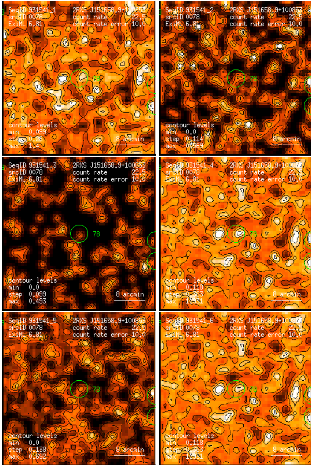
Figure 78: RASS 931541: detection 0078: band rate images, Gaussian filter: (1) PSPC channels 11 – 41, (2) 52 – 90, (3) 91 – 201, (4) 11 – 235, (5) 52 – 201, (6) 11 – 201. Broad band rates in counts/ks. Band rate contour levels in counts/ks/arcmin 2 .
