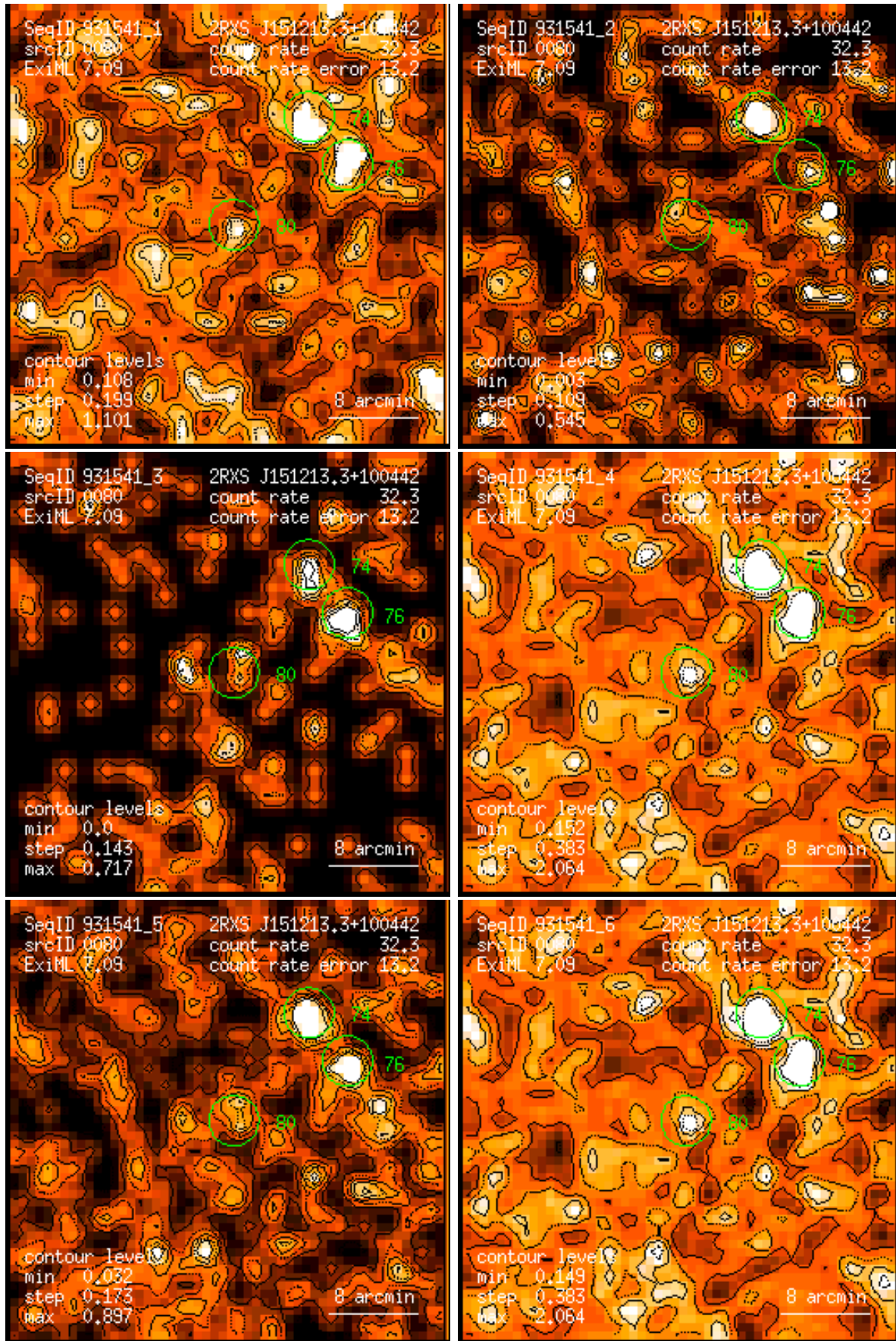
Figure 80: RASS 931541: detection 0080: band rate images, Gaussian filter: (1) PSPC channels 11 – 41, (2) 52 – 90, (3) 91 – 201, (4) 11 – 235, (5) 52 – 201, (6) 11 – 201. Broad band rates in counts/ks. Band rate contour levels in counts/ks/arcmin 2 .
