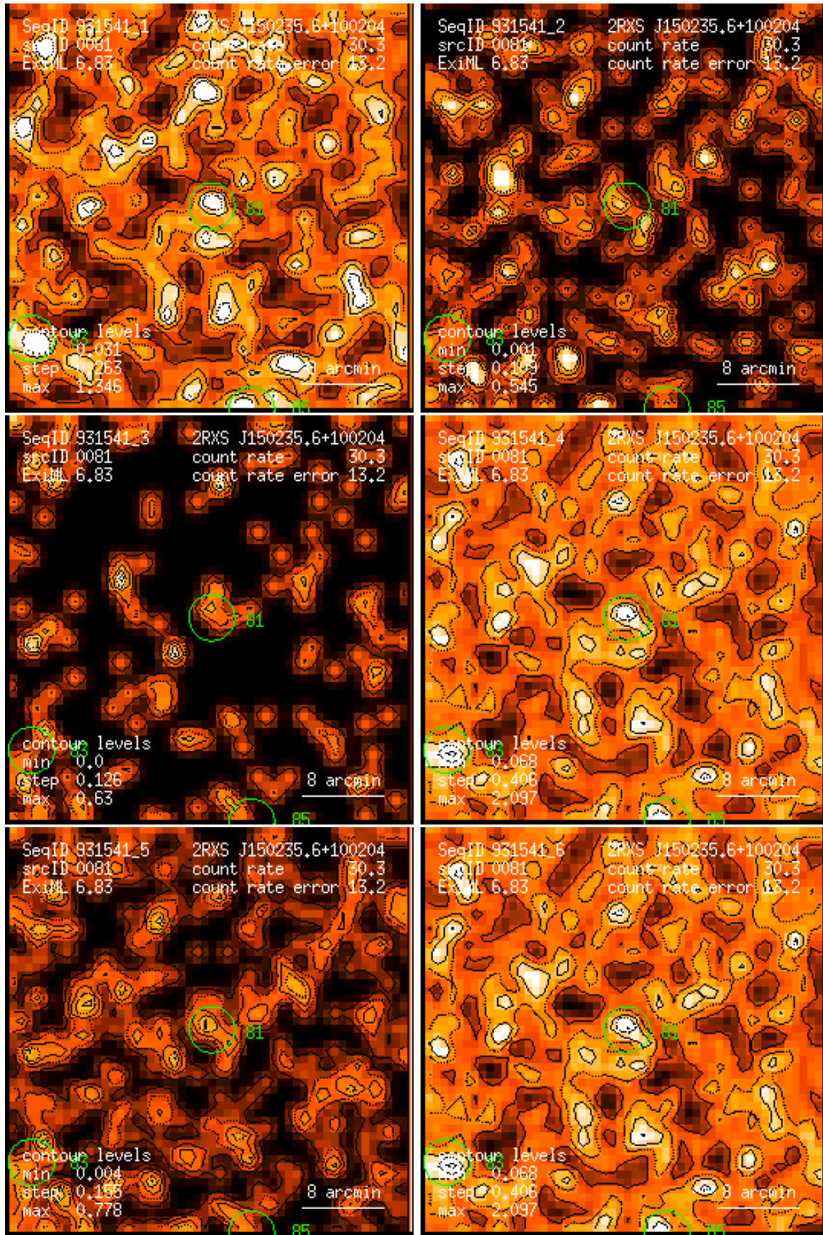
Figure 81: RASS 931541: detection 0081: band rate images, Gaussian filter: (1) PSPC channels 11 – 41, (2) 52 – 90, (3) 91 – 201, (4) 11 – 235, (5) 52 – 201, (6) 11 – 201. Broad band rates in counts/ks. Band rate contour levels in counts/ks/arcmin 2 .
