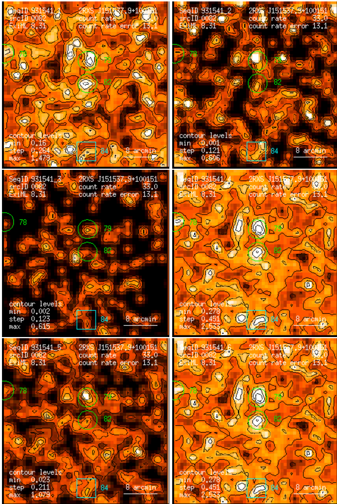
Figure 82: RASS 931541: detection 0082: band rate images, Gaussian filter: (1) PSPC channels 11 – 41, (2) 52 – 90, (3) 91 – 201, (4) 11 – 235, (5) 52 – 201, (6) 11 – 201. Broad band rates in counts/ks. Band rate contour levels in counts/ks/arcmin 2 .
