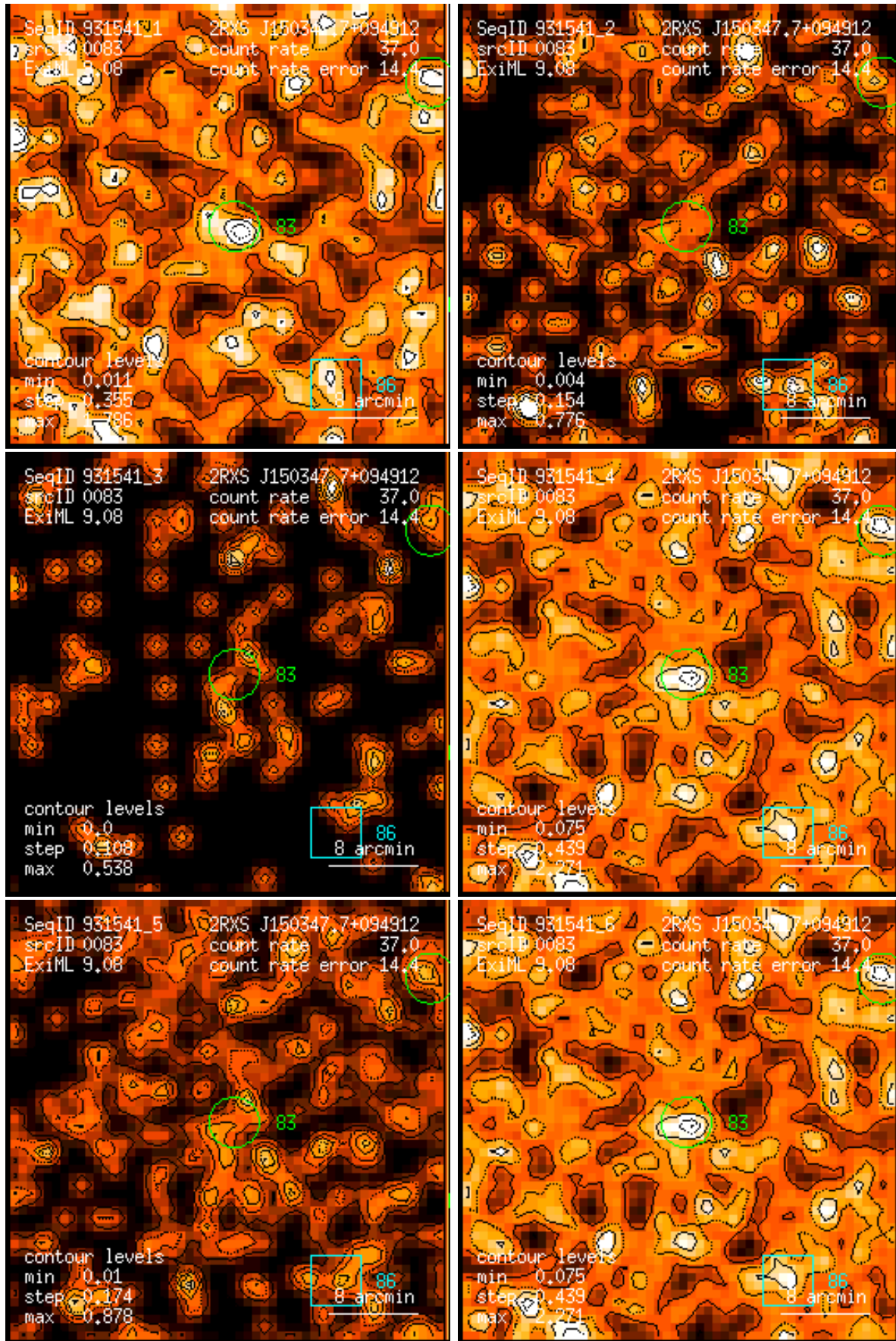
Figure 83: RASS 931541: detection 0083: band rate images, Gaussian filter: (1) PSPC channels 11 – 41, (2) 52 – 90, (3) 91 – 201, (4) 11 – 235, (5) 52 – 201, (6) 11 – 201. Broad band rates in counts/ks. Band rate contour levels in counts/ks/arcmin 2 .
