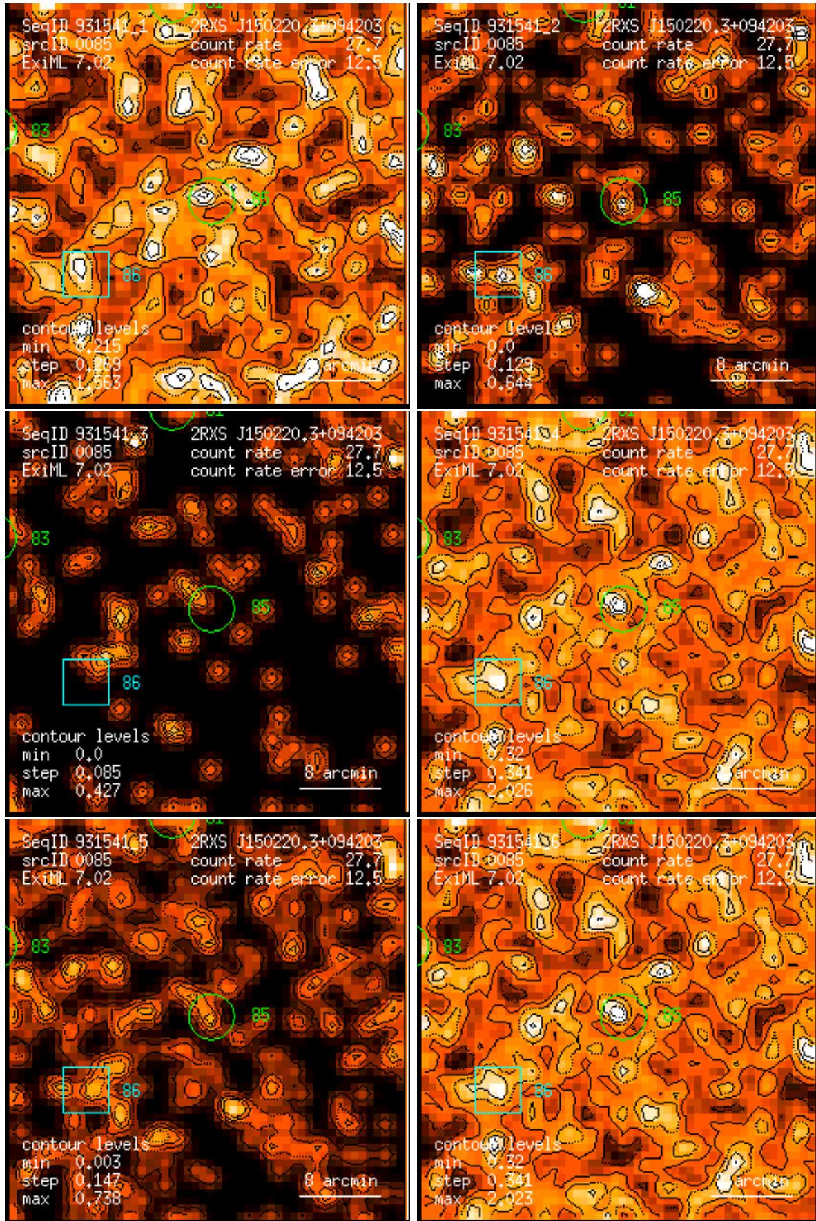
Figure 85: RASS 931541: detection 0085: band rate images, Gaussian filter: (1) PSPC channels 11 – 41, (2) 52 – 90, (3) 91 – 201, (4) 11 – 235, (5) 52 – 201, (6) 11 – 201. Broad band rates in counts/ks. Band rate contour levels in counts/ks/arcmin 2 .
