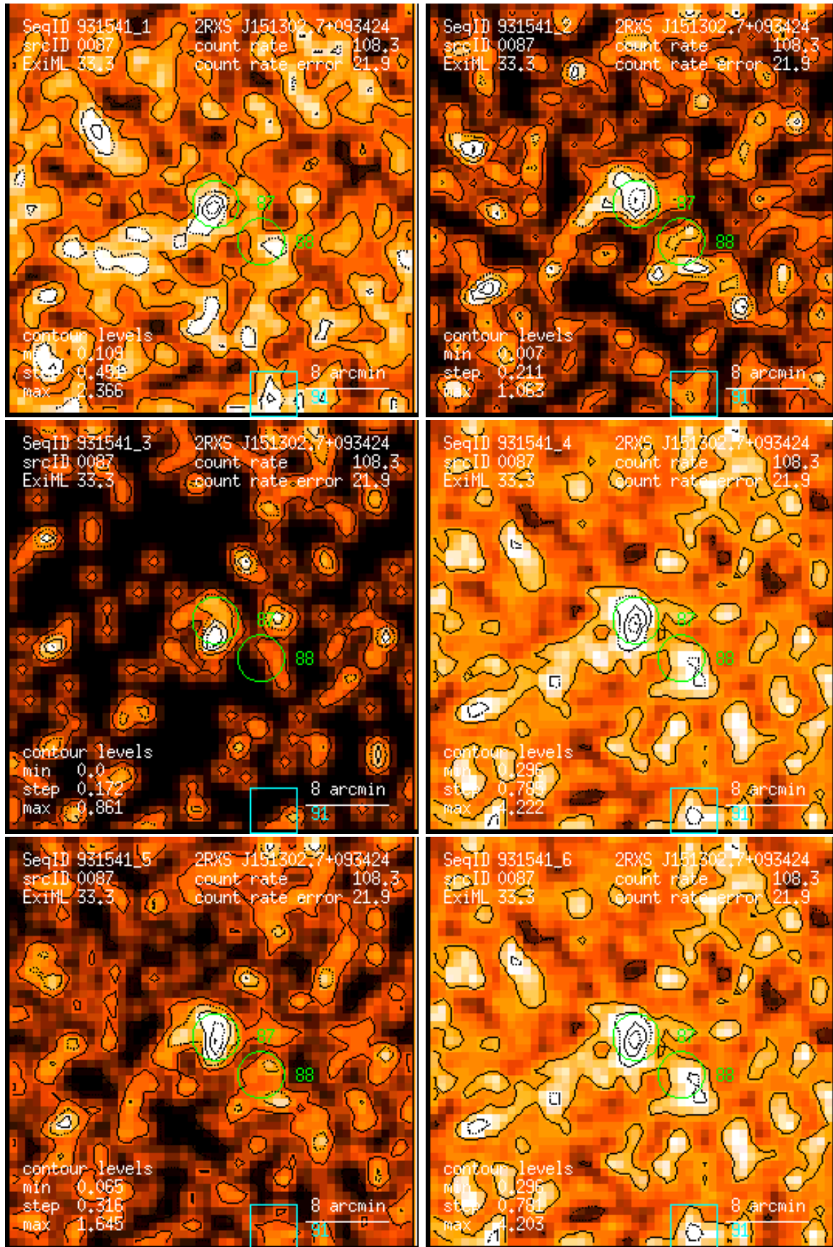
Figure 87: RASS 931541: detection 0087: band rate images, Gaussian filter: (1) PSPC channels 11 – 41, (2) 52 – 90, (3) 91 – 201, (4) 11 – 235, (5) 52 – 201, (6) 11 – 201. Broad band rates in counts/ks. Band rate contour levels in counts/ks/arcmin 2 .
