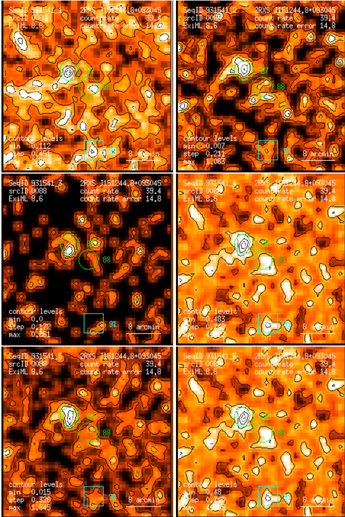
Figure 88: RASS 931541: detection 0088: band rate images, Gaussian filter: (1) PSPC channels 11 – 41, (2) 52 – 90, (3) 91 – 201, (4) 11 – 235, (5) 52 – 201, (6) 11 – 201. Broad band rates in counts/ks. Band rate contour levels in counts/ks/arcmin 2 .
