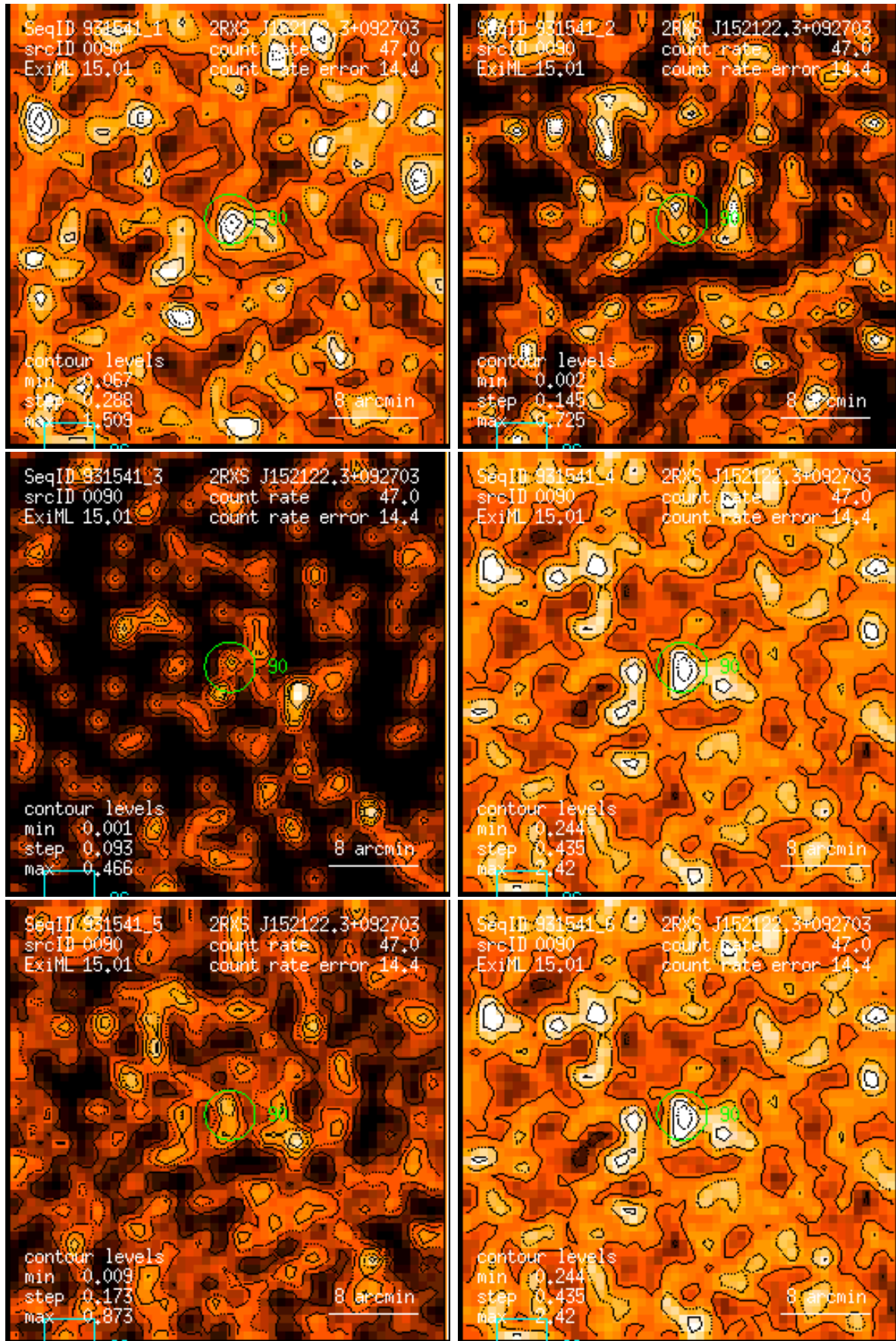
Figure 90: RASS 931541: detection 0090: band rate images, Gaussian filter: (1) PSPC channels 11 – 41, (2) 52 – 90, (3) 91 – 201, (4) 11 – 235, (5) 52 – 201, (6) 11 – 201. Broad band rates in counts/ks. Band rate contour levels in counts/ks/arcmin 2 .
