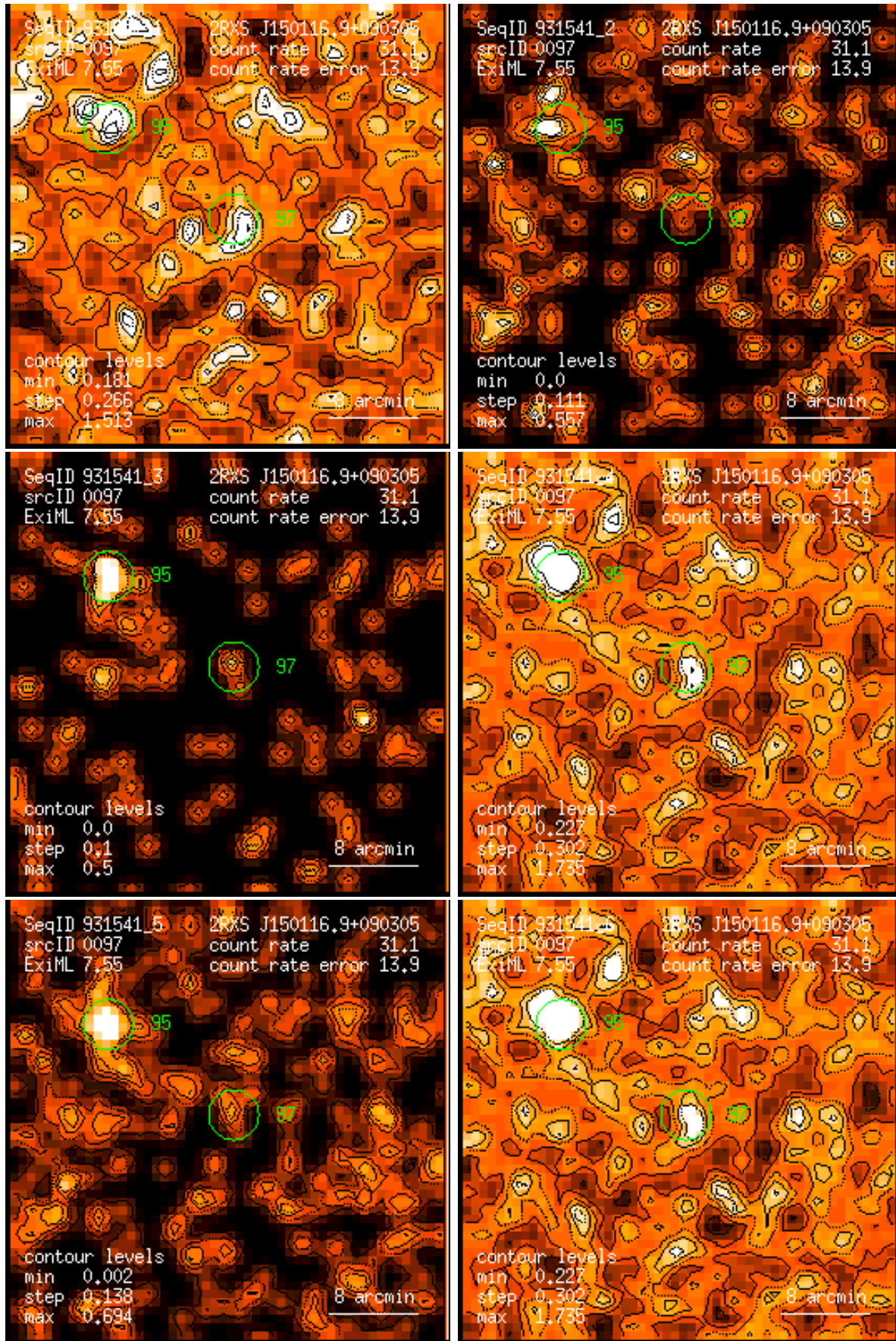
Figure 97: RASS 931541: detection 0097: band rate images, Gaussian filter: (1) PSPC channels 11 – 41, (2) 52 – 90, (3) 91 – 201, (4) 11 – 235, (5) 52 – 201, (6) 11 – 201. Broad band rates in counts/ks. Band rate contour levels in counts/ks/arcmin 2 .
