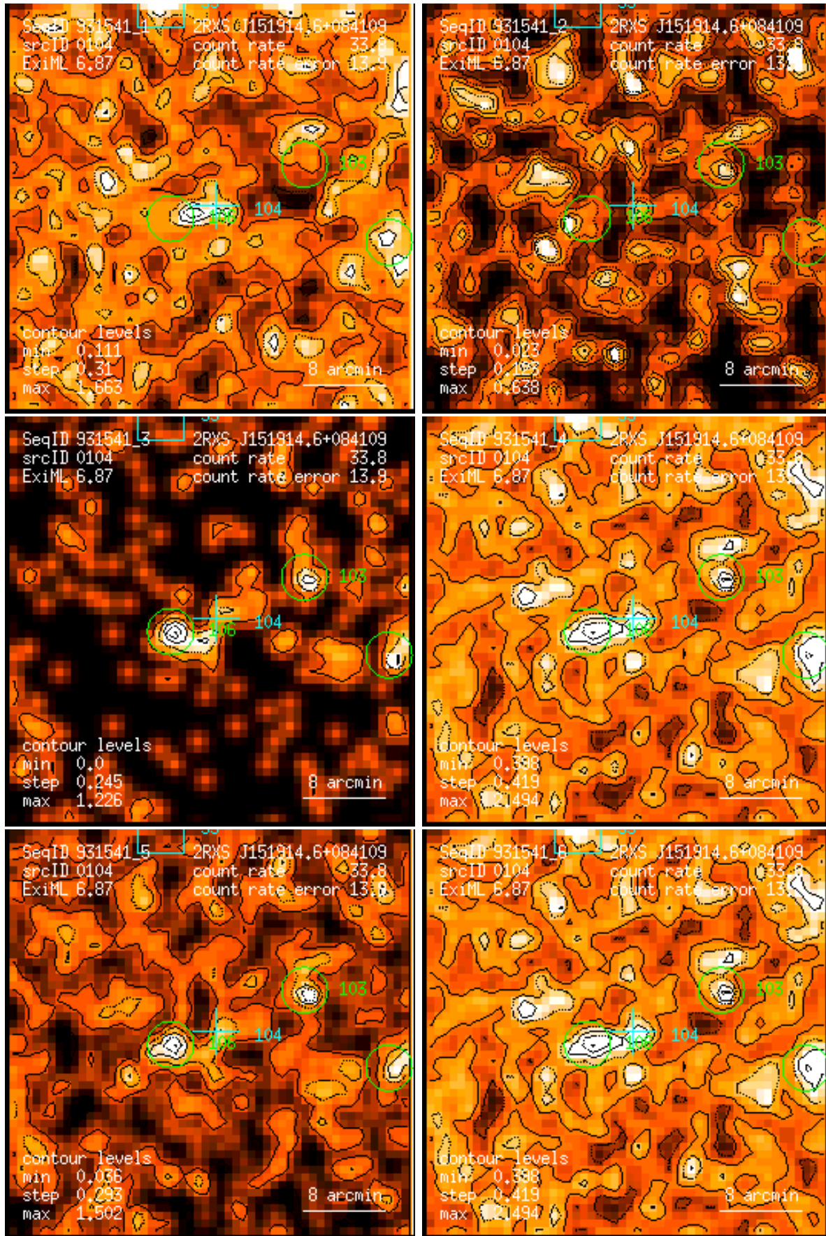
Figure 104: RASS 931541: detection 0104: band rate images, Gaussian filter: (1) PSPC channels 11 – 41, (2) 52 – 90, (3) 91 – 201, (4) 11 – 235, (5) 52 – 201, (6) 11 – 201. Broad band rates in counts/ks. Band rate contour levels in counts/ks/arcmin 2 .
