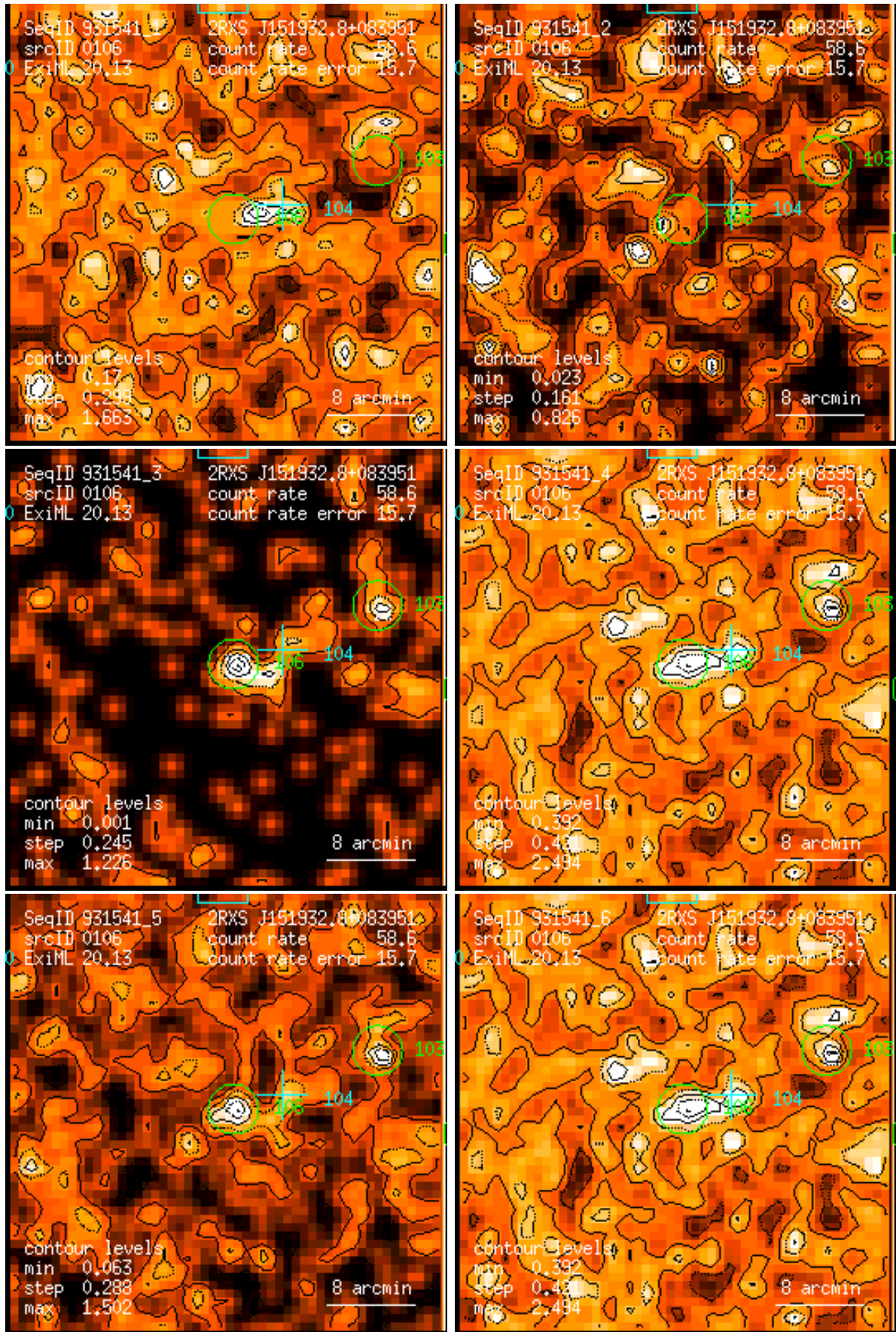
Figure 106: RASS 931541: detection 0106: band rate images, Gaussian filter: (1) PSPC channels 11 – 41, (2) 52 – 90, (3) 91 – 201, (4) 11 – 235, (5) 52 – 201, (6) 11 – 201. Broad band rates in counts/ks. Band rate contour levels in counts/ks/arcmin 2 .
