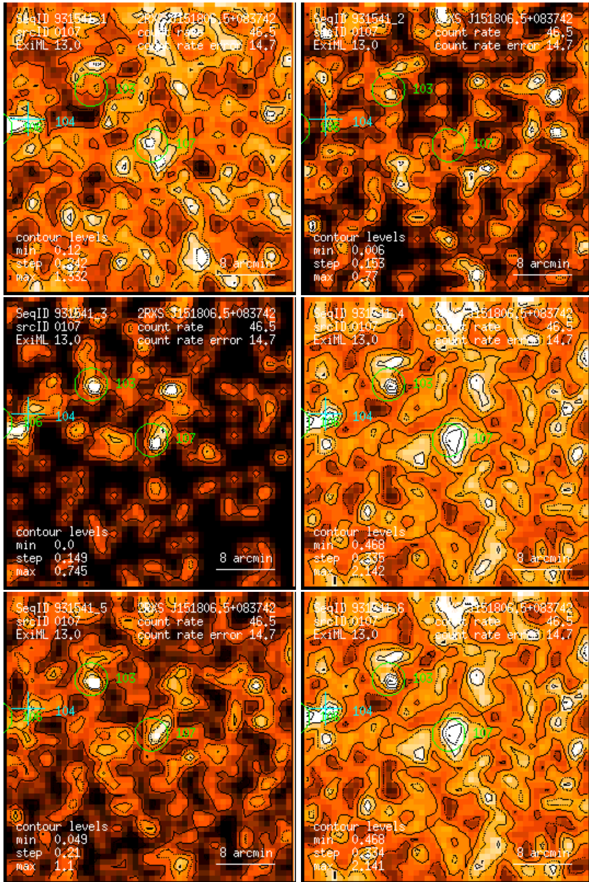
Figure 107: RASS 931541: detection 0107: band rate images, Gaussian filter: (1) PSPC channels 11 – 41, (2) 52 – 90, (3) 91 – 201, (4) 11 – 235, (5) 52 – 201, (6) 11 – 201. Broad band rates in counts/ks. Band rate contour levels in counts/ks/arcmin 2 .
