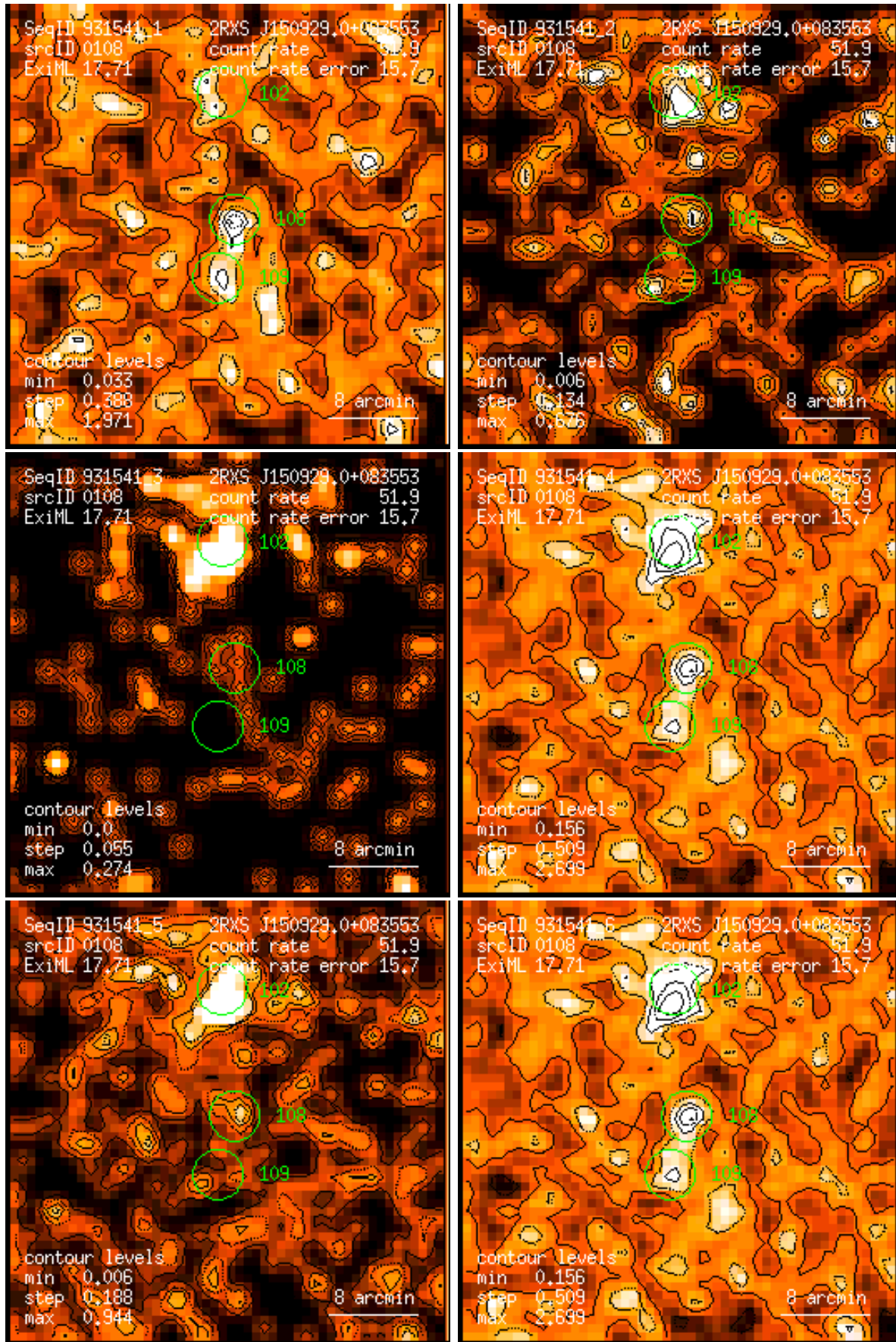
Figure 108: RASS 931541: detection 0108: band rate images, Gaussian filter: (1) PSPC channels 11 – 41, (2) 52 – 90, (3) 91 – 201, (4) 11 – 235, (5) 52 – 201, (6) 11 – 201. Broad band rates in counts/ks. Band rate contour levels in counts/ks/arcmin 2 .
