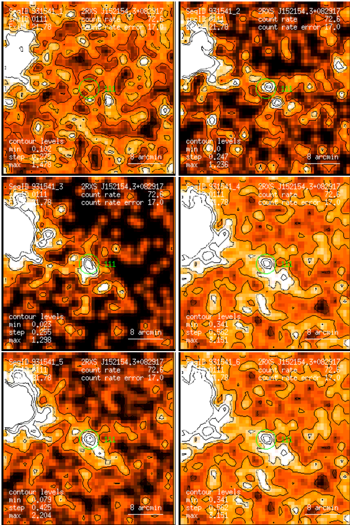
Figure 111: RASS 931541: detection 0111: band rate images, Gaussian filter: (1) PSPC channels 11 – 41, (2) 52 – 90, (3) 91 – 201, (4) 11 – 235, (5) 52 – 201, (6) 11 – 201. Broad band rates in counts/ks. Band rate contour levels in counts/ks/arcmin 2 .
