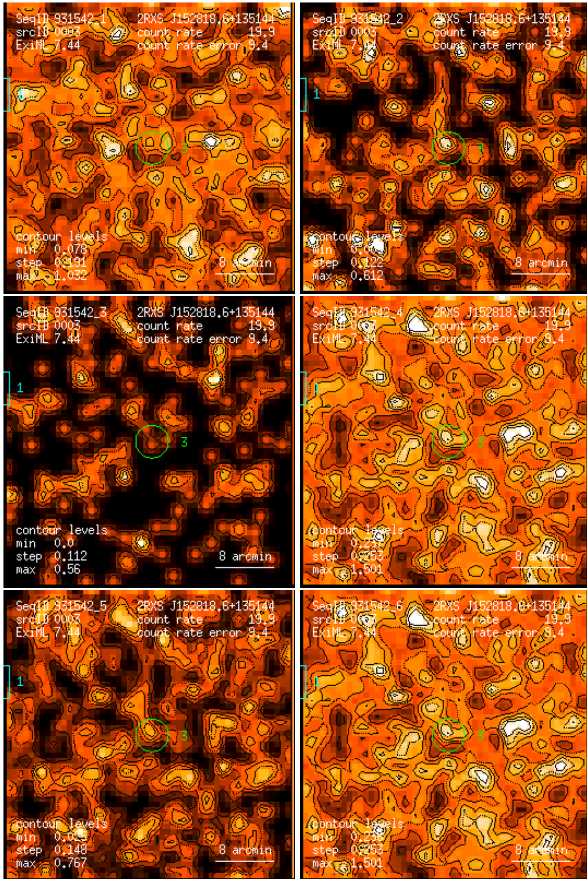
Figure 3: RASS 931542: detection 0003: band rate images, Gaussian filter: (1) PSPC channels 11 – 41, (2) 52 – 90, (3) 91 – 201, (4) 11 – 235, (5) 52 – 201, (6) 11 – 201. Broad band rates in counts/ks. Band rate contour levels in counts/ks/arcmin 2 .
