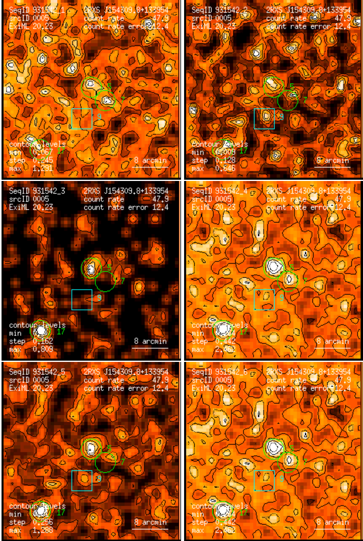
Figure 5: RASS 931542: detection 0005: band rate images, Gaussian filter: (1) PSPC channels 11 – 41, (2) 52 – 90, (3) 91 – 201, (4) 11 – 235, (5) 52 – 201, (6) 11 – 201. Broad band rates in counts/ks. Band rate contour levels in counts/ks/arcmin 2 .
