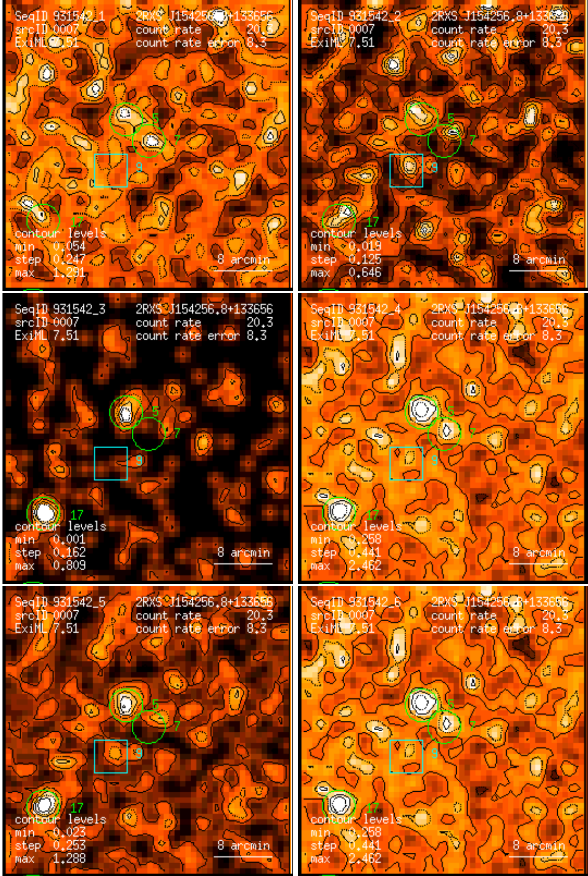
Figure 7: RASS 931542: detection 0007: band rate images, Gaussian filter: (1) PSPC channels 11 – 41, (2) 52 – 90, (3) 91 – 201, (4) 11 – 235, (5) 52 – 201, (6) 11 – 201. Broad band rates in counts/ks. Band rate contour levels in counts/ks/arcmin 2 .
