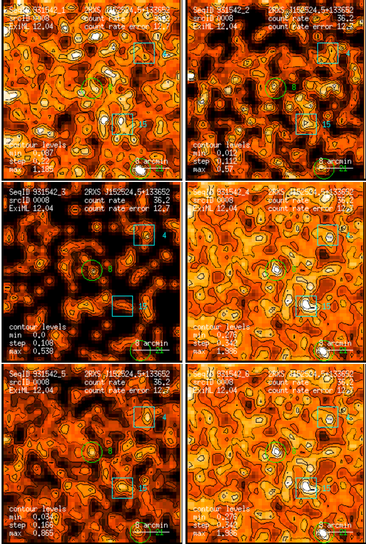
Figure 8: RASS 931542: detection 0008: band rate images, Gaussian filter: (1) PSPC channels 11 – 41, (2) 52 – 90, (3) 91 – 201, (4) 11 – 235, (5) 52 – 201, (6) 11 – 201. Broad band rates in counts/ks. Band rate contour levels in counts/ks/arcmin 2 .
