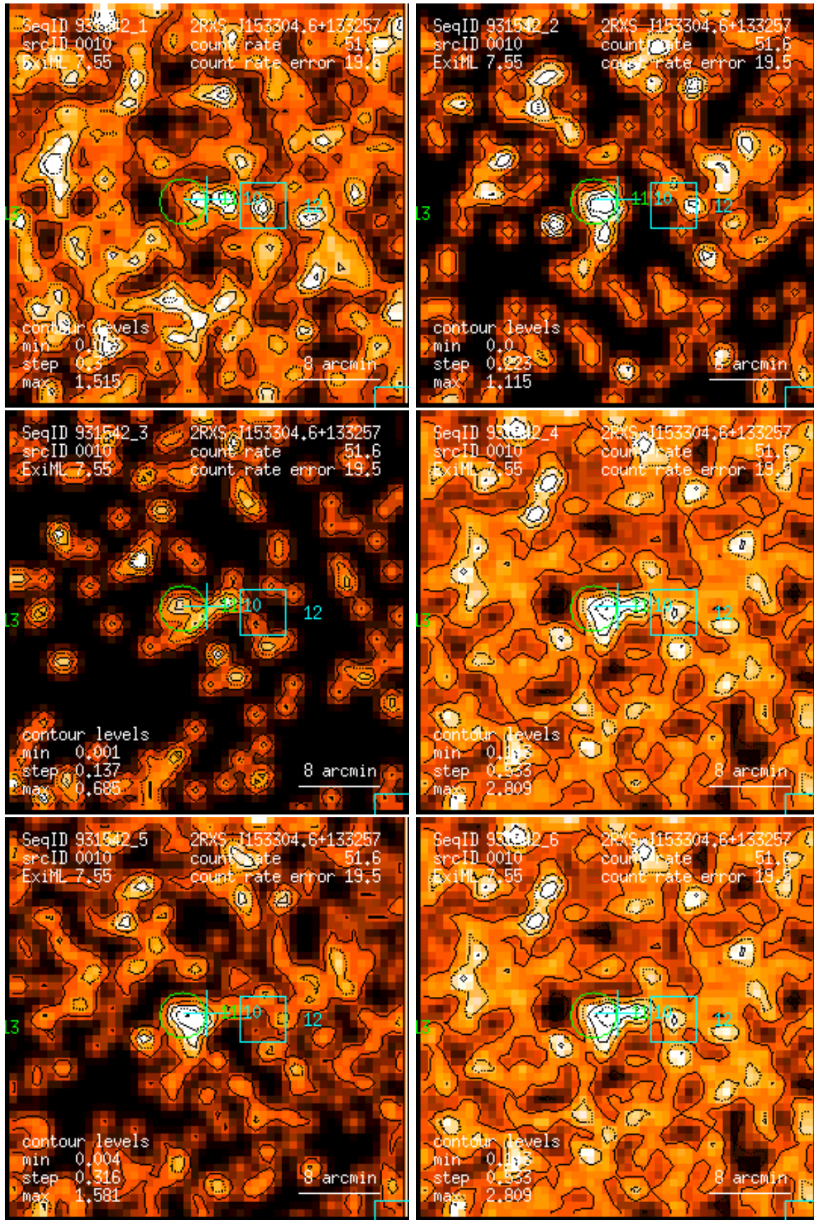
Figure 10: RASS 931542: detection 0010: band rate images, Gaussian filter: (1) PSPC channels 11 – 41, (2) 52 – 90, (3) 91 – 201, (4) 11 – 235, (5) 52 – 201, (6) 11 – 201. Broad band rates in counts/ks. Band rate contour levels in counts/ks/arcmin 2 .
