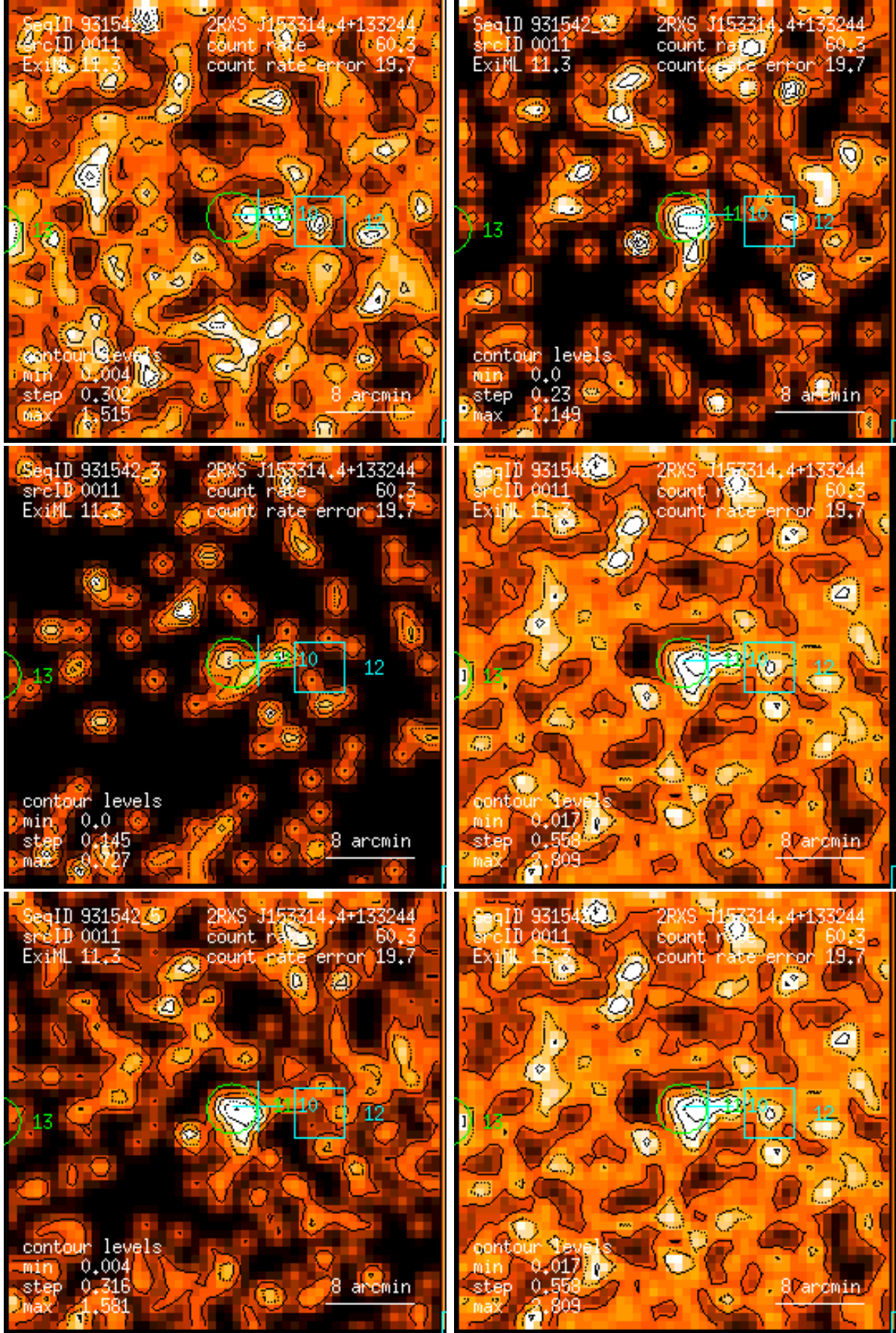
Figure 11: RASS 931542: detection 0011: band rate images, Gaussian filter: (1) PSPC channels 11 – 41, (2) 52 – 90, (3) 91 – 201, (4) 11 – 235, (5) 52 – 201, (6) 11 – 201. Broad band rates in counts/ks. Band rate contour levels in counts/ks/arcmin 2 .
