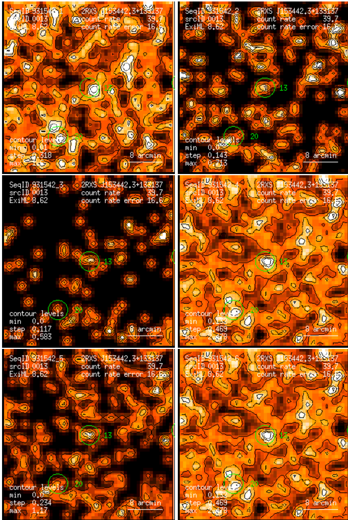
Figure 13: RASS 931542: detection 0013: band rate images, Gaussian filter: (1) PSPC channels 11 – 41, (2) 52 – 90, (3) 91 – 201, (4) 11 – 235, (5) 52 – 201, (6) 11 – 201. Broad band rates in counts/ks. Band rate contour levels in counts/ks/arcmin 2 .
