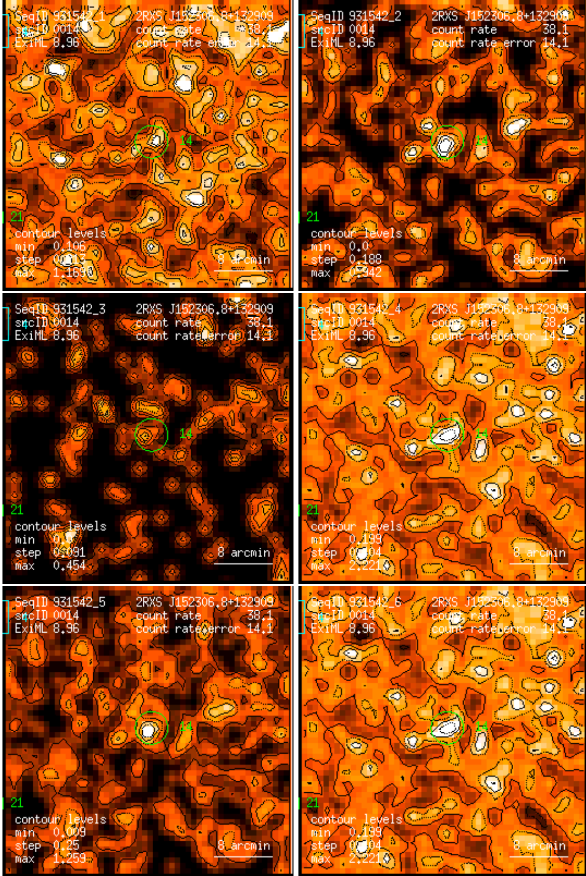
Figure 14: RASS 931542: detection 0014: band rate images, Gaussian filter: (1) PSPC channels 11 – 41, (2) 52 – 90, (3) 91 – 201, (4) 11 – 235, (5) 52 – 201, (6) 11 – 201. Broad band rates in counts/ks. Band rate contour levels in counts/ks/arcmin 2 .
