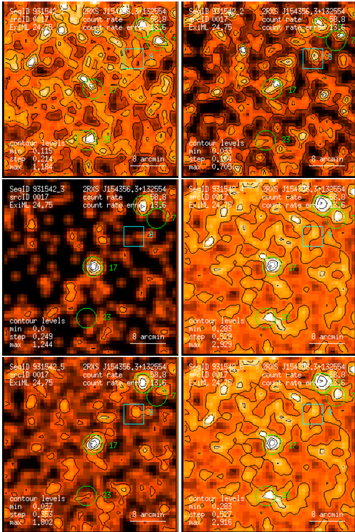
Figure 17: RASS 931542: detection 0017: band rate images, Gaussian filter: (1) PSPC channels 11 – 41, (2) 52 – 90, (3) 91 – 201, (4) 11 – 235, (5) 52 – 201, (6) 11 – 201. Broad band rates in counts/ks. Band rate contour levels in counts/ks/arcmin 2 .
