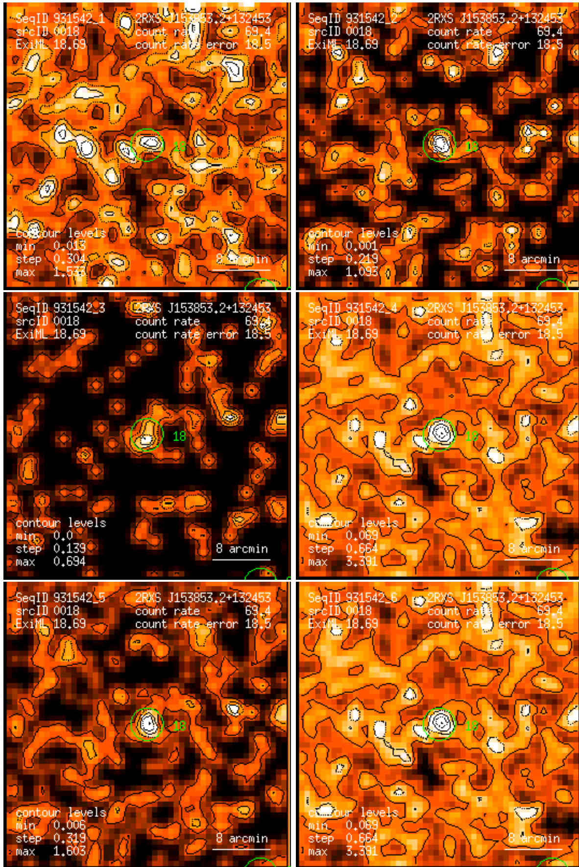
Figure 18: RASS 931542: detection 0018: band rate images, Gaussian filter: (1) PSPC channels 11 – 41, (2) 52 – 90, (3) 91 – 201, (4) 11 – 235, (5) 52 – 201, (6) 11 – 201. Broad band rates in counts/ks. Band rate contour levels in counts/ks/arcmin 2 .
