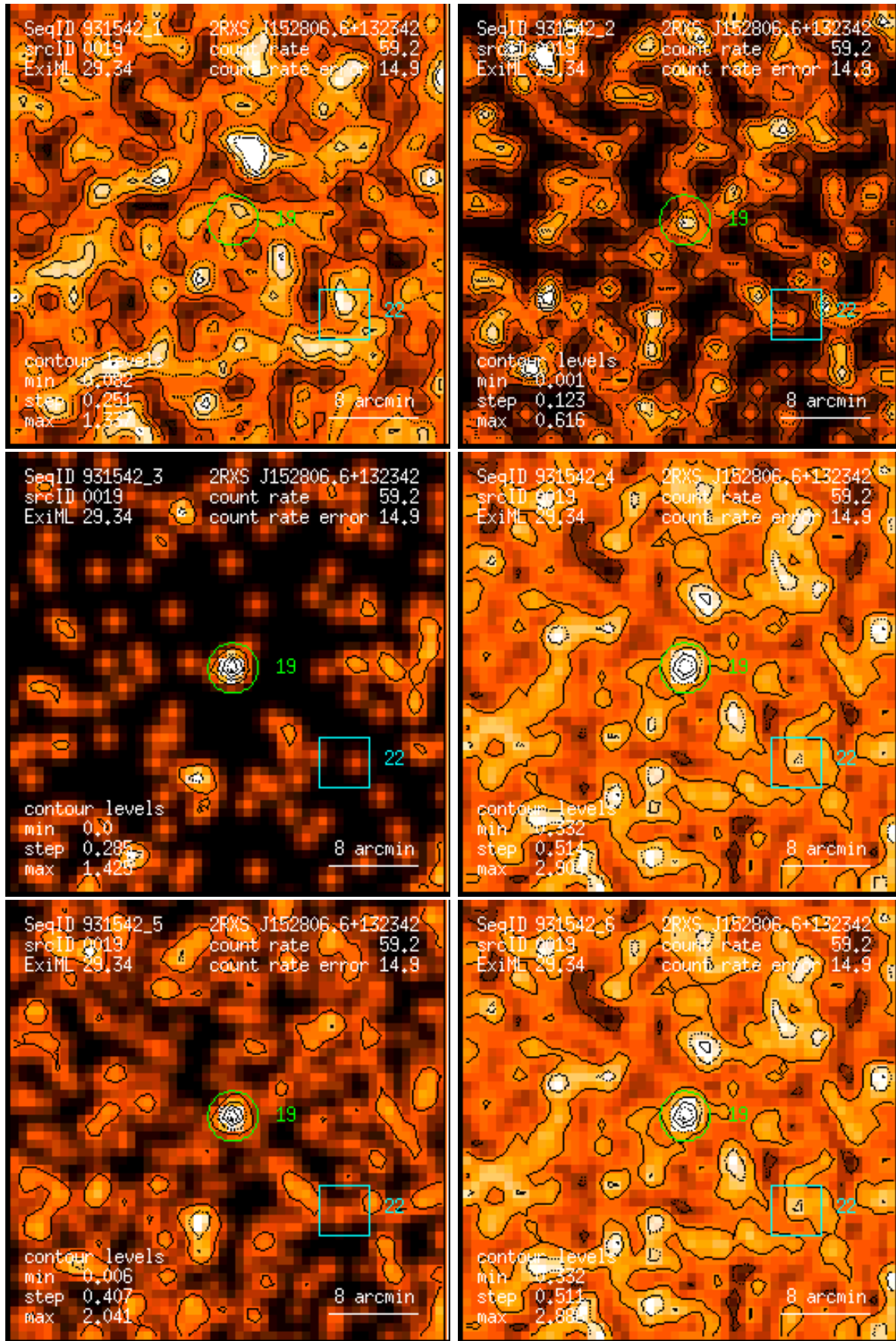
Figure 19: RASS 931542: detection 0019: band rate images, Gaussian filter: (1) PSPC channels 11 – 41, (2) 52 – 90, (3) 91 – 201, (4) 11 – 235, (5) 52 – 201, (6) 11 – 201. Broad band rates in counts/ks. Band rate contour levels in counts/ks/arcmin 2 .
