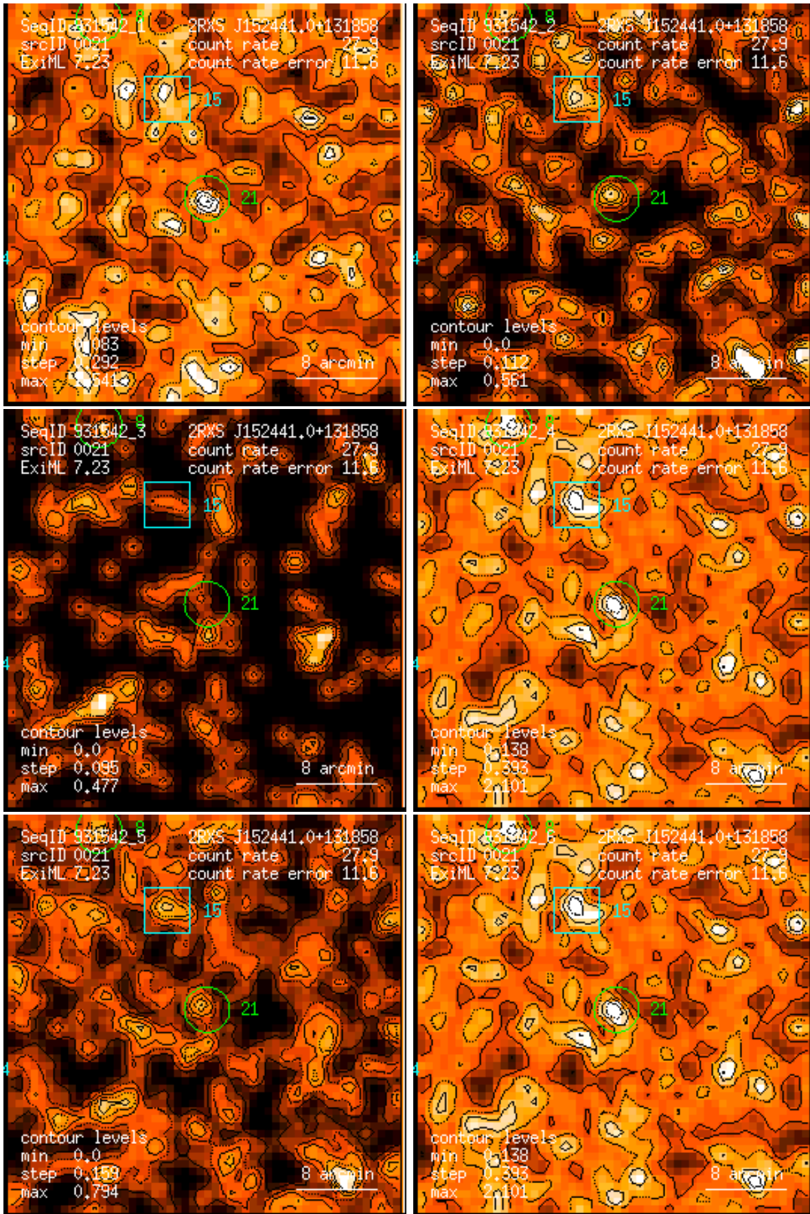
Figure 21: RASS 931542: detection 0021: band rate images, Gaussian filter: (1) PSPC channels 11 – 41, (2) 52 – 90, (3) 91 – 201, (4) 11 – 235, (5) 52 – 201, (6) 11 – 201. Broad band rates in counts/ks. Band rate contour levels in counts/ks/arcmin 2 .
