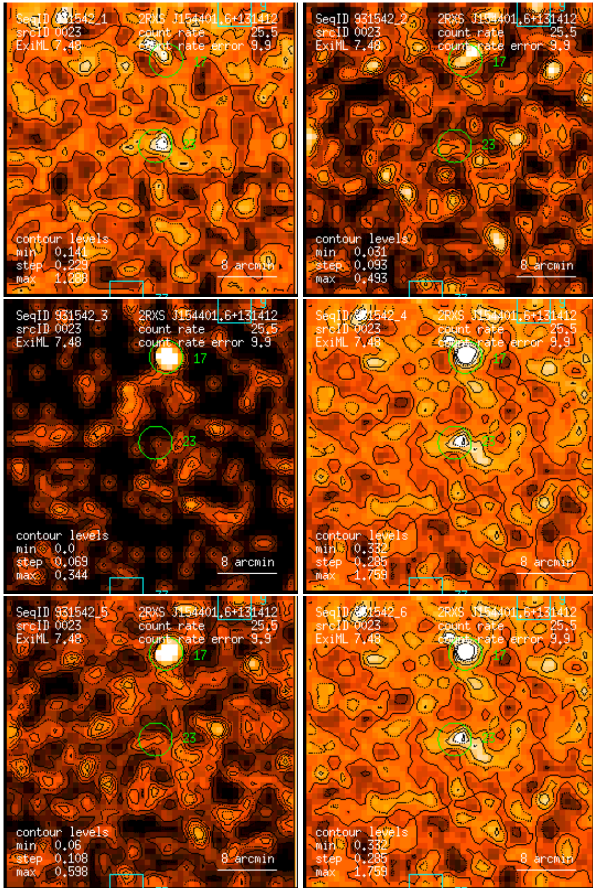
Figure 23: RASS 931542: detection 0023: band rate images, Gaussian filter: (1) PSPC channels 11 – 41, (2) 52 – 90, (3) 91 – 201, (4) 11 – 235, (5) 52 – 201, (6) 11 – 201. Broad band rates in counts/ks. Band rate contour levels in counts/ks/arcmin 2 .
