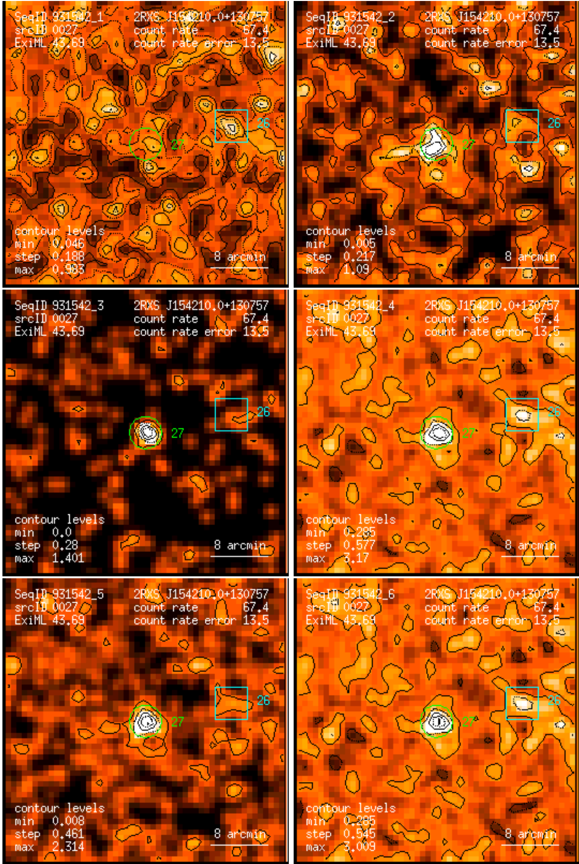
Figure 27: RASS 931542: detection 0027: band rate images, Gaussian filter: (1) PSPC channels 11 – 41, (2) 52 – 90, (3) 91 – 201, (4) 11 – 235, (5) 52 – 201, (6) 11 – 201. Broad band rates in counts/ks. Band rate contour levels in counts/ks/arcmin 2 .
