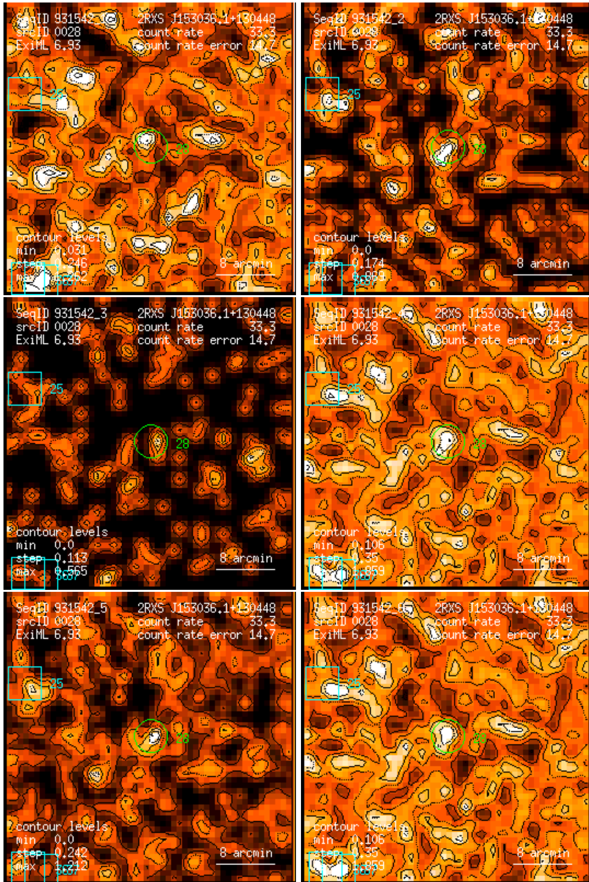
Figure 28: RASS 931542: detection 0028: band rate images, Gaussian filter: (1) PSPC channels 11 – 41, (2) 52 – 90, (3) 91 – 201, (4) 11 – 235, (5) 52 – 201, (6) 11 – 201. Broad band rates in counts/ks. Band rate contour levels in counts/ks/arcmin 2 .
