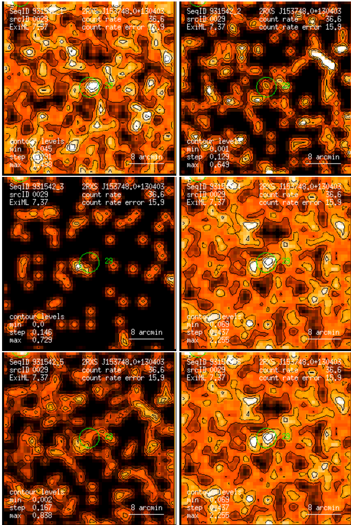
Figure 29: RASS 931542: detection 0029: band rate images, Gaussian filter: (1) PSPC channels 11 – 41, (2) 52 – 90, (3) 91 – 201, (4) 11 – 235, (5) 52 – 201, (6) 11 – 201. Broad band rates in counts/ks. Band rate contour levels in counts/ks/arcmin 2 .
