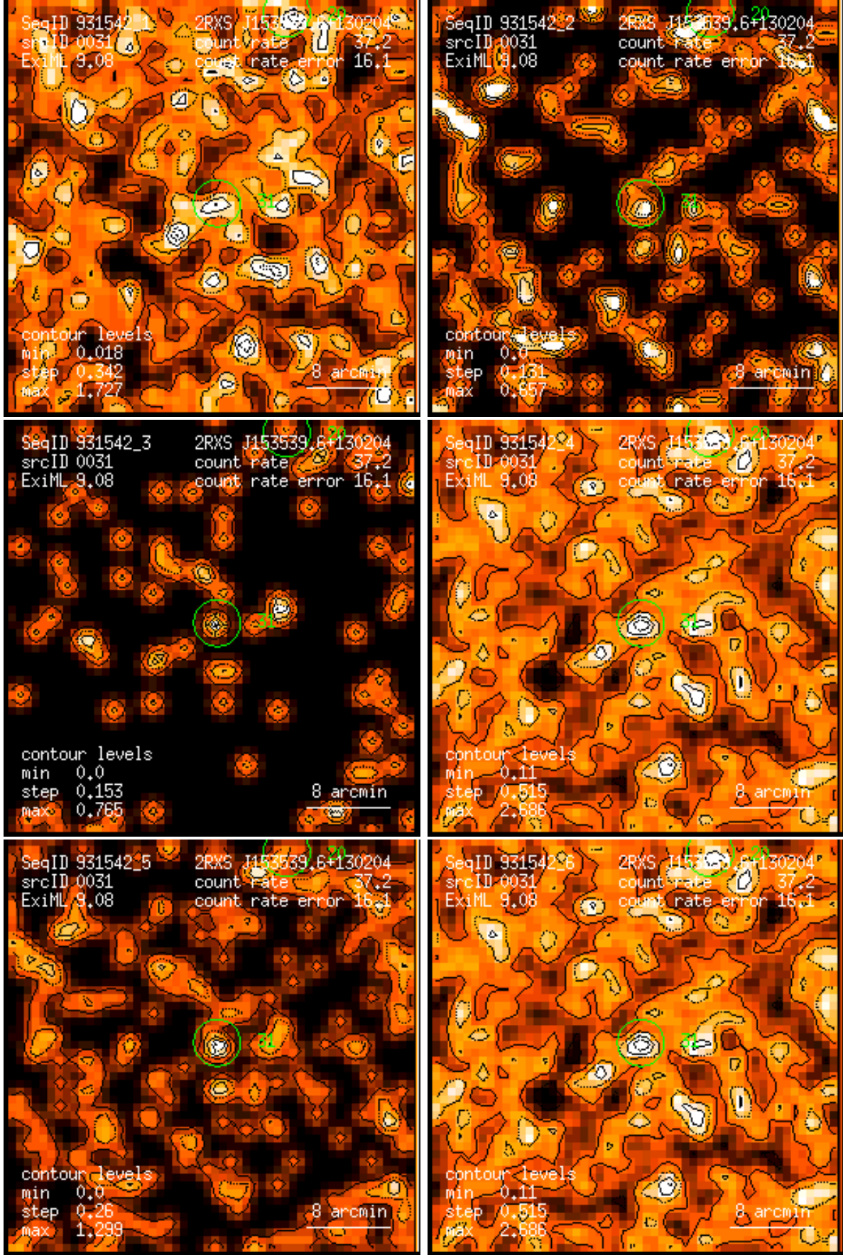
Figure 31: RASS 931542: detection 0031: band rate images, Gaussian filter: (1) PSPC channels 11 – 41, (2) 52 – 90, (3) 91 – 201, (4) 11 – 235, (5) 52 – 201, (6) 11 – 201. Broad band rates in counts/ks. Band rate contour levels in counts/ks/arcmin 2 .
